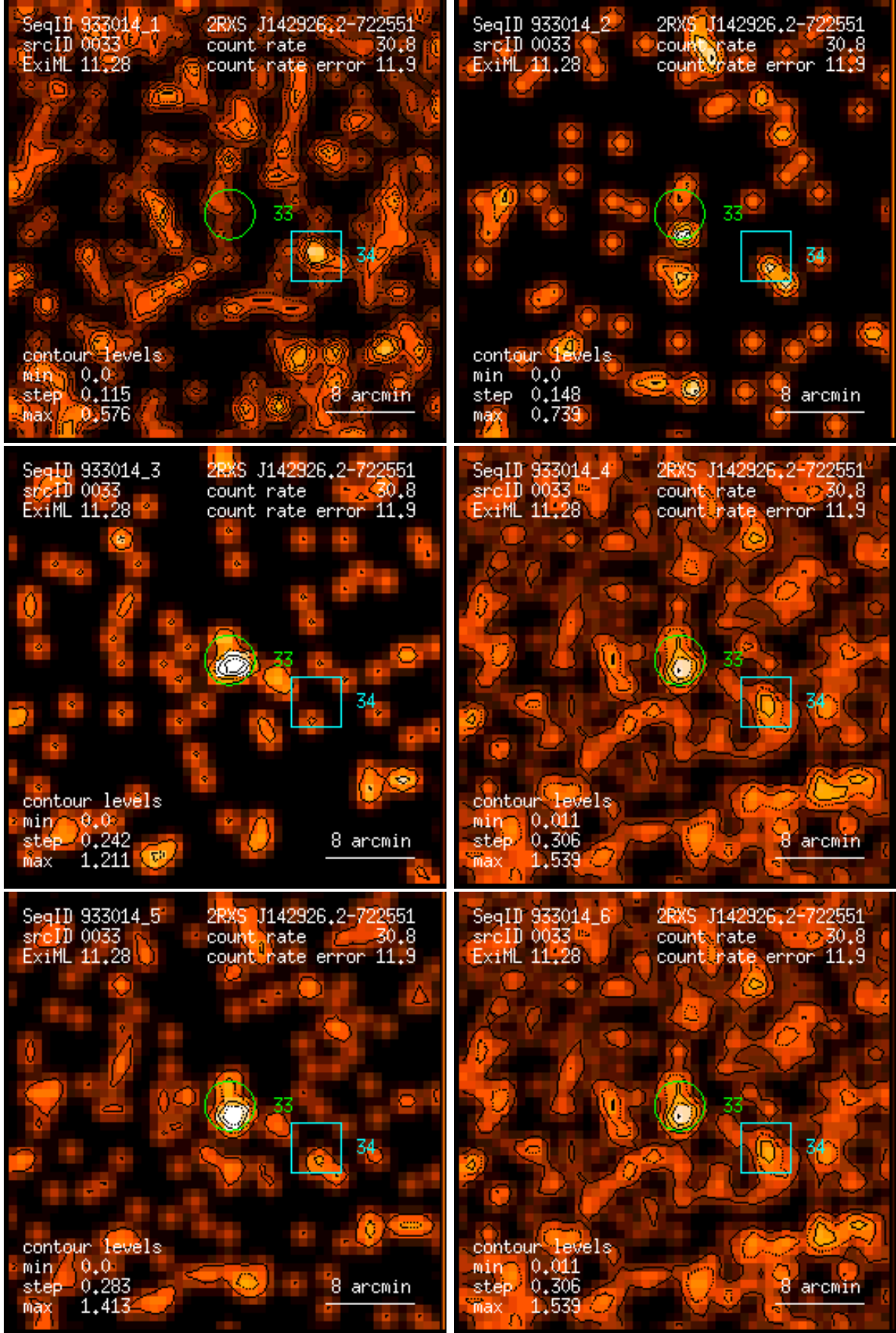
Figure 33: RASS 933014: detection 0033: band rate images, Gaussian filter: (1) PSPC channels 11 – 41, (2) 52 – 90, (3) 91 – 201, (4) 11 – 235, (5) 52 – 201, (6) 11 – 201. Broad band rates in counts/ks. Band rate contour levels in counts/ks/arcmin 2 .
