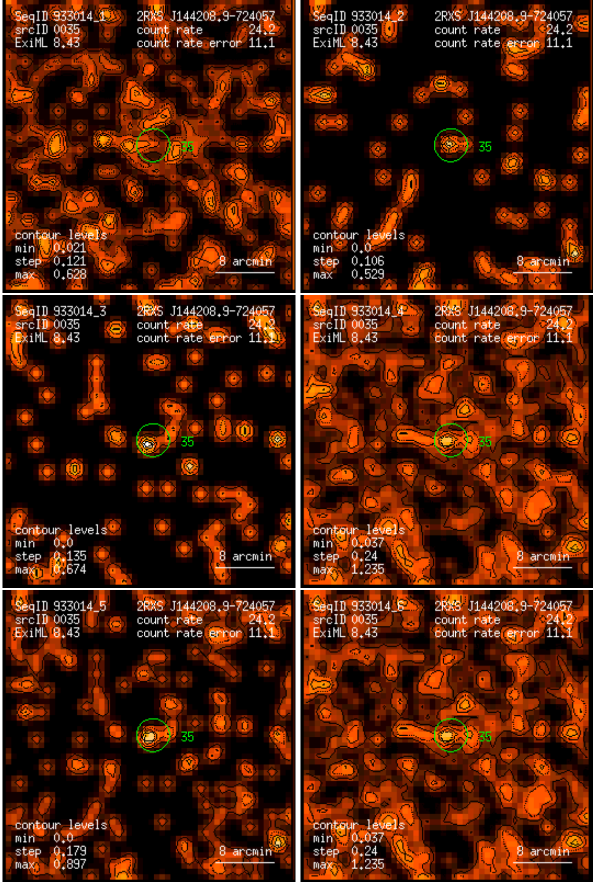
Figure 35: RASS 933014: detection 0035: band rate images, Gaussian filter: (1) PSPC channels 11 – 41, (2) 52 – 90, (3) 91 – 201, (4) 11 – 235, (5) 52 – 201, (6) 11 – 201. Broad band rates in counts/ks. Band rate contour levels in counts/ks/arcmin 2 .
