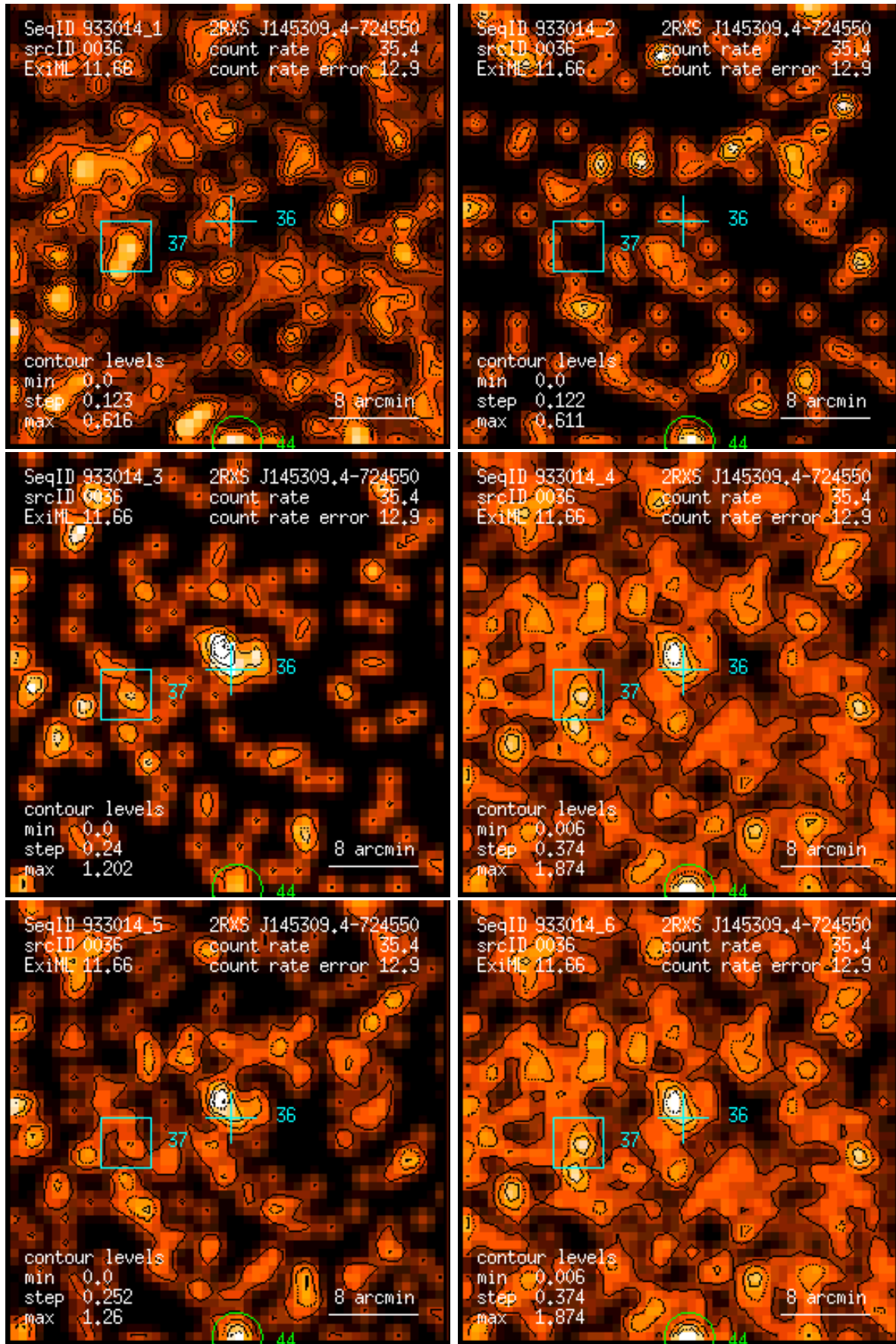
Figure 36: RASS 933014: detection 0036: band rate images, Gaussian filter: (1) PSPC channels 11 – 41, (2) 52 – 90, (3) 91 – 201, (4) 11 – 235, (5) 52 – 201, (6) 11 – 201. Broad band rates in counts/ks. Band rate contour levels in counts/ks/arcmin 2 .
