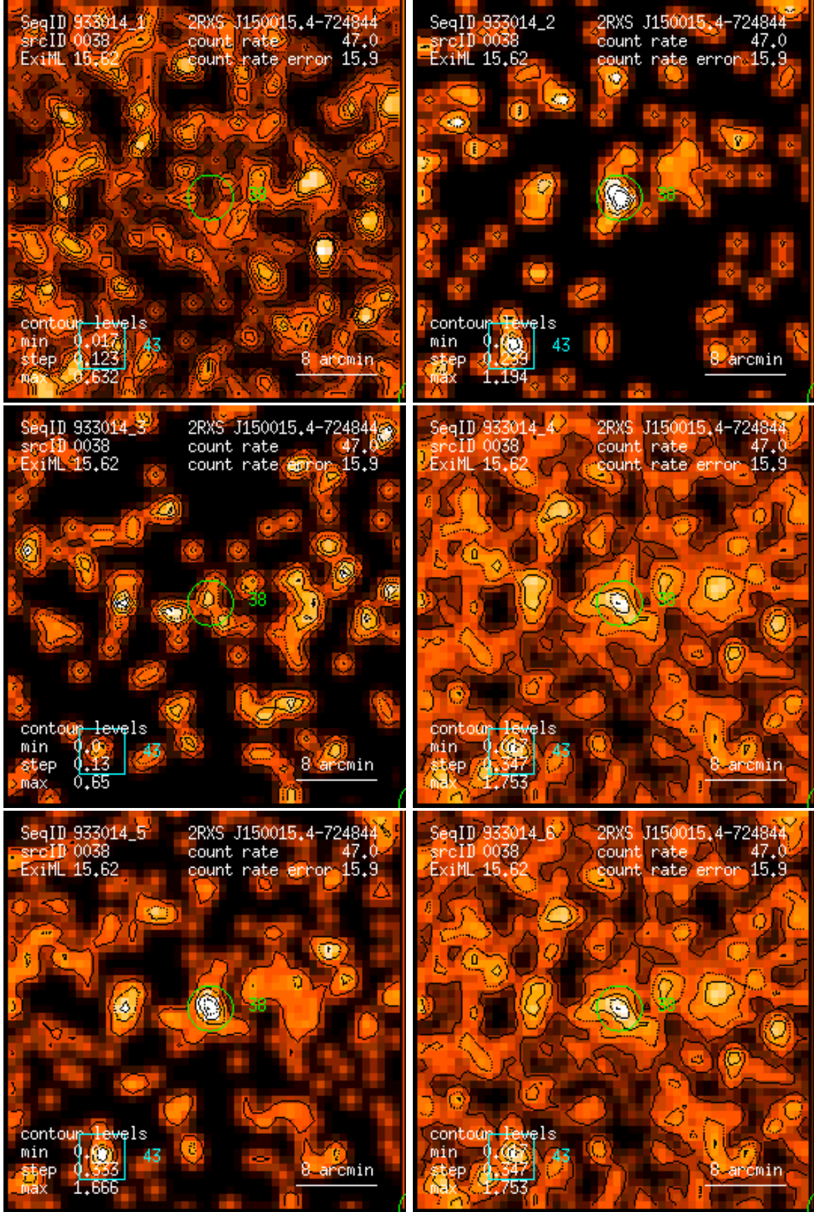
Figure 38: RASS 933014: detection 0038: band rate images, Gaussian filter: (1) PSPC channels 11 – 41, (2) 52 – 90, (3) 91 – 201, (4) 11 – 235, (5) 52 – 201, (6) 11 – 201. Broad band rates in counts/ks. Band rate contour levels in counts/ks/arcmin 2 .
