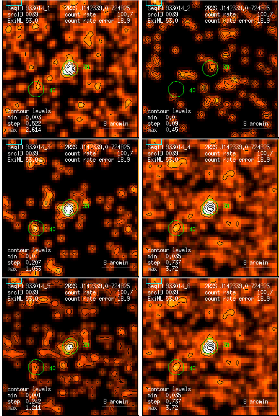
Figure 39: RASS 933014: detection 0039: band rate images, Gaussian filter: (1) PSPC channels 11 – 41, (2) 52 – 90, (3) 91 – 201, (4) 11 – 235, (5) 52 – 201, (6) 11 – 201. Broad band rates in counts/ks. Band rate contour levels in counts/ks/arcmin 2 .
