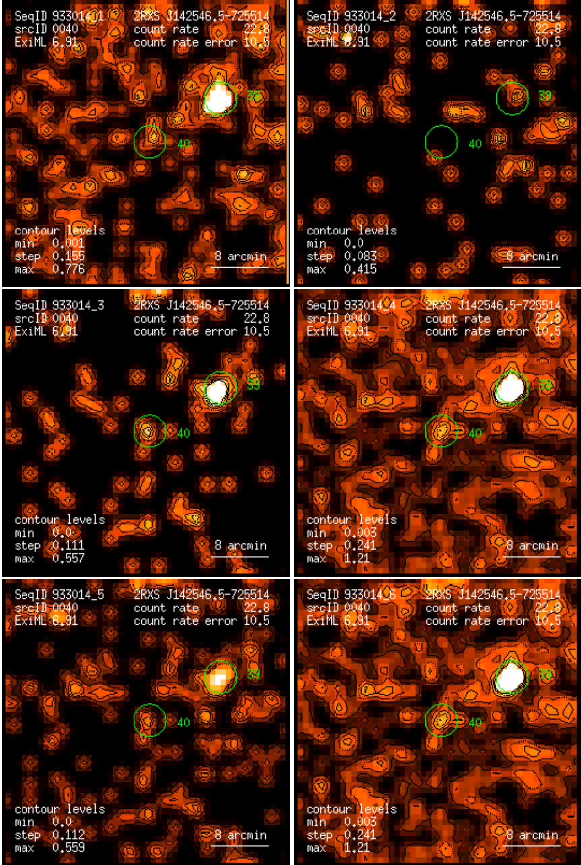
Figure 40: RASS 933014: detection 0040: band rate images, Gaussian filter: (1) PSPC channels 11 – 41, (2) 52 – 90, (3) 91 – 201, (4) 11 – 235, (5) 52 – 201, (6) 11 – 201. Broad band rates in counts/ks. Band rate contour levels in counts/ks/arcmin 2 .
