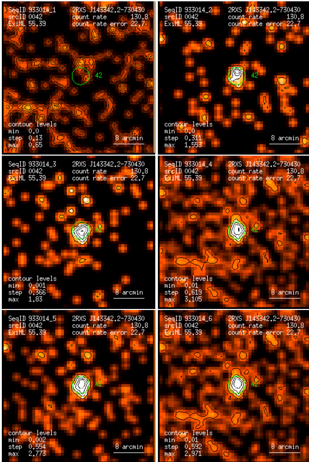
Figure 42: RASS 933014: detection 0042: band rate images, Gaussian filter: (1) PSPC channels 11 – 41, (2) 52 – 90, (3) 91 – 201, (4) 11 – 235, (5) 52 – 201, (6) 11 – 201. Broad band rates in counts/ks. Band rate contour levels in counts/ks/arcmin 2 .
