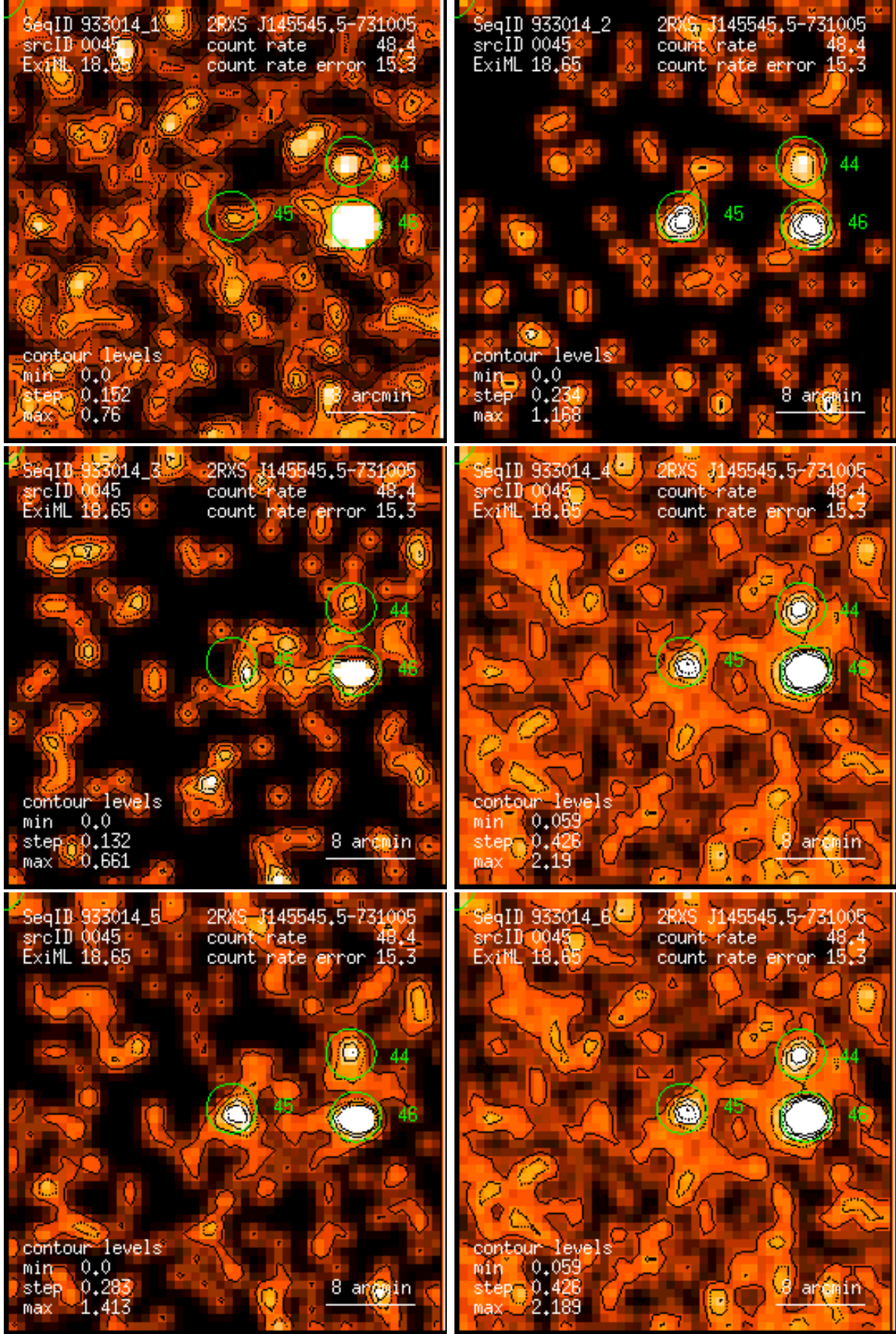
Figure 45: RASS 933014: detection 0045: band rate images, Gaussian filter: (1) PSPC channels 11 – 41, (2) 52 – 90, (3) 91 – 201, (4) 11 – 235, (5) 52 – 201, (6) 11 – 201. Broad band rates in counts/ks. Band rate contour levels in counts/ks/arcmin 2 .
