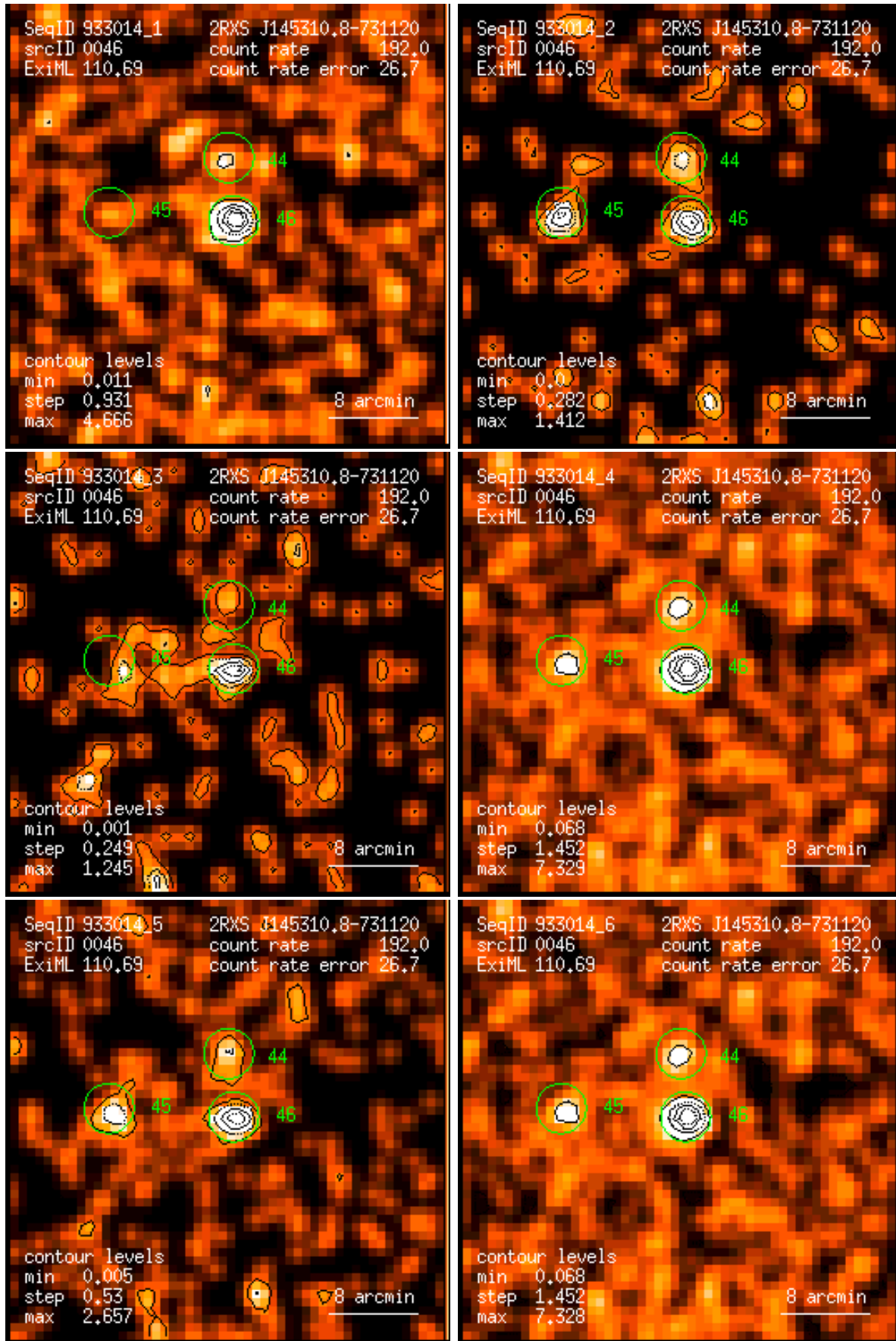
Figure 46: RASS 933014: detection 0046: band rate images, Gaussian filter: (1) PSPC channels 11 – 41, (2) 52 – 90, (3) 91 – 201, (4) 11 – 235, (5) 52 – 201, (6) 11 – 201. Broad band rates in counts/ks. Band rate contour levels in counts/ks/arcmin 2 .
