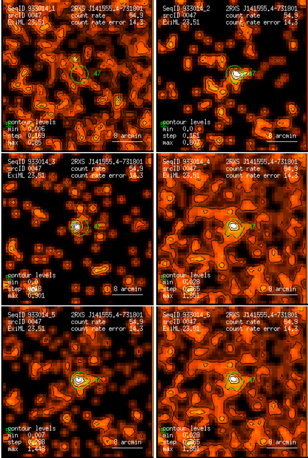
Figure 47: RASS 933014: detection 0047: band rate images, Gaussian filter: (1) PSPC channels 11 – 41, (2) 52 – 90, (3) 91 – 201, (4) 11 – 235, (5) 52 – 201, (6) 11 – 201. Broad band rates in counts/ks. Band rate contour levels in counts/ks/arcmin 2 .
