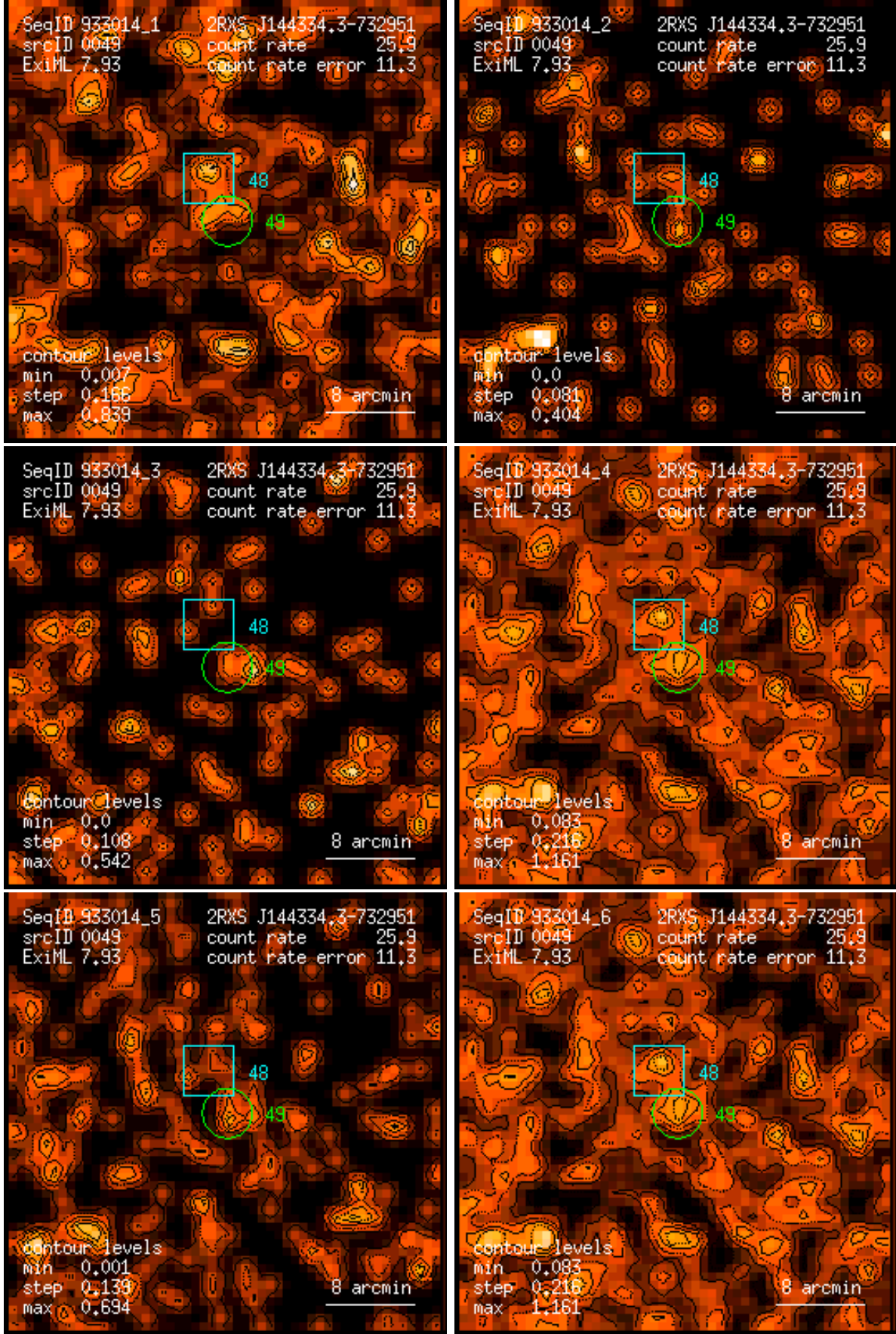
Figure 49: RASS 933014: detection 0049: band rate images, Gaussian filter: (1) PSPC channels 11 – 41, (2) 52 – 90, (3) 91 – 201, (4) 11 – 235, (5) 52 – 201, (6) 11 – 201. Broad band rates in counts/ks. Band rate contour levels in counts/ks/arcmin 2 .
