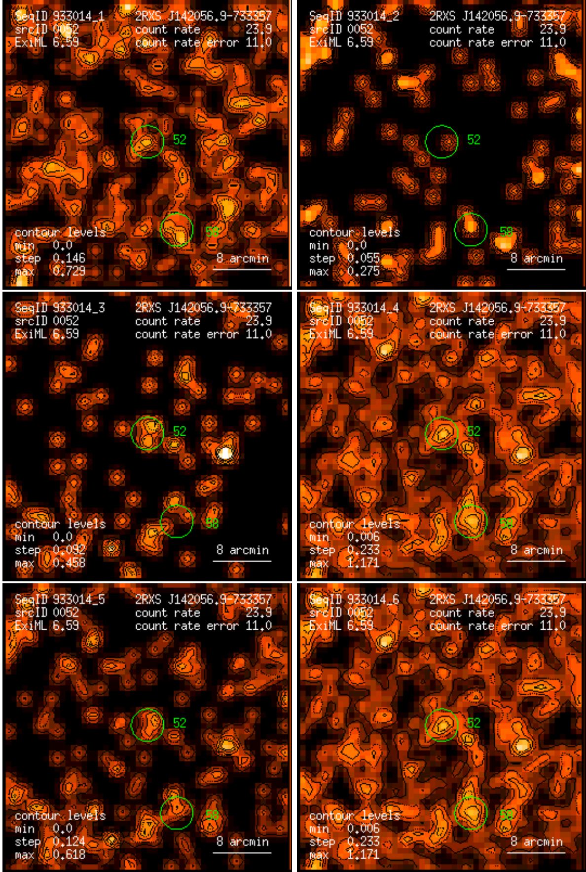
Figure 52: RASS 933014: detection 0052: band rate images, Gaussian filter: (1) PSPC channels 11 – 41, (2) 52 – 90, (3) 91 – 201, (4) 11 – 235, (5) 52 – 201, (6) 11 – 201. Broad band rates in counts/ks. Band rate contour levels in counts/ks/arcmin 2 .
