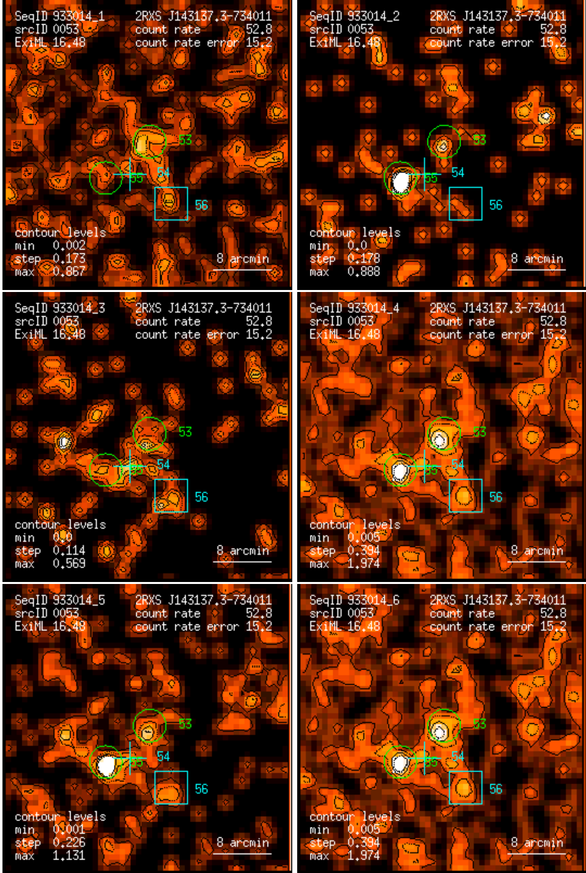
Figure 53: RASS 933014: detection 0053: band rate images, Gaussian filter: (1) PSPC channels 11 – 41, (2) 52 – 90, (3) 91 – 201, (4) 11 – 235, (5) 52 – 201, (6) 11 – 201. Broad band rates in counts/ks. Band rate contour levels in counts/ks/arcmin 2 .
