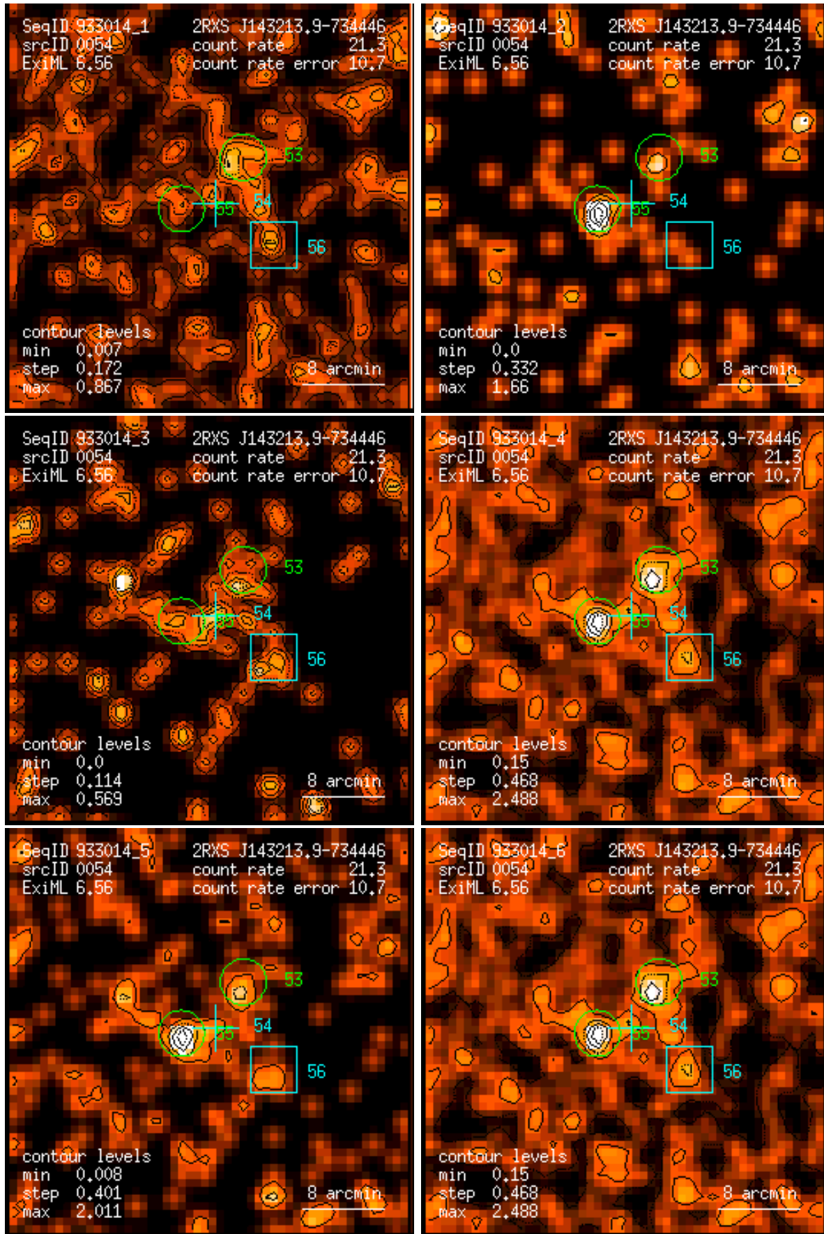
Figure 54: RASS 933014: detection 0054: band rate images, Gaussian filter: (1) PSPC channels 11 – 41, (2) 52 – 90, (3) 91 – 201, (4) 11 – 235, (5) 52 – 201, (6) 11 – 201. Broad band rates in counts/ks. Band rate contour levels in counts/ks/arcmin 2 .
