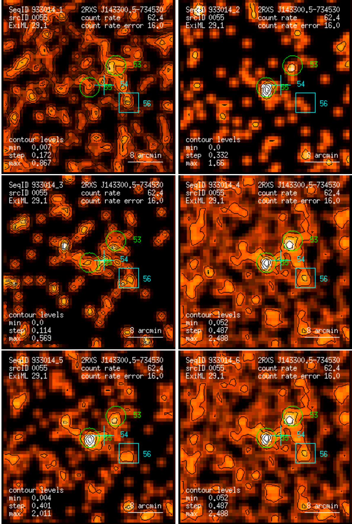
Figure 55: RASS 933014: detection 0055: band rate images, Gaussian filter: (1) PSPC channels 11 – 41, (2) 52 – 90, (3) 91 – 201, (4) 11 – 235, (5) 52 – 201, (6) 11 – 201. Broad band rates in counts/ks. Band rate contour levels in counts/ks/arcmin 2 .
