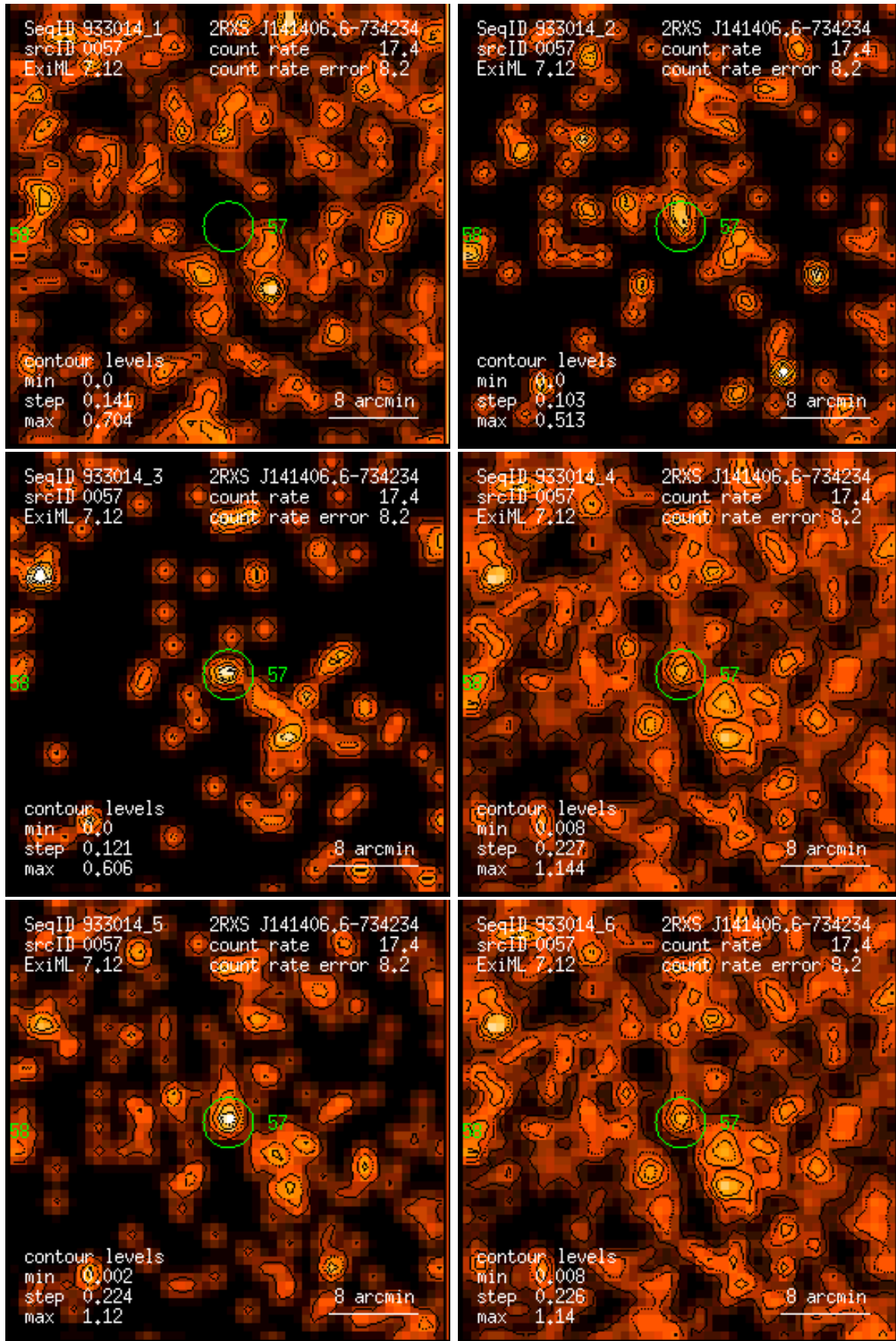
Figure 57: RASS 933014: detection 0057: band rate images, Gaussian filter: (1) PSPC channels 11 – 41, (2) 52 – 90, (3) 91 – 201, (4) 11 – 235, (5) 52 – 201, (6) 11 – 201. Broad band rates in counts/ks. Band rate contour levels in counts/ks/arcmin 2 .
