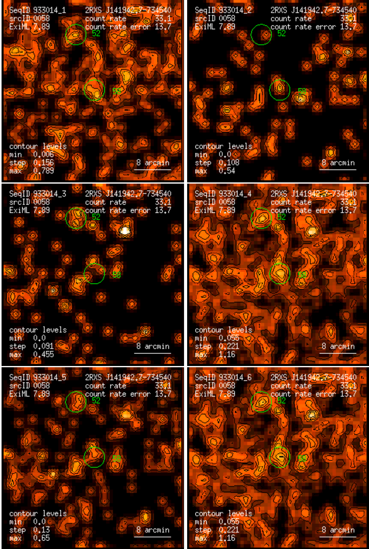
Figure 58: RASS 933014: detection 0058: band rate images, Gaussian filter: (1) PSPC channels 11 – 41, (2) 52 – 90, (3) 91 – 201, (4) 11 – 235, (5) 52 – 201, (6) 11 – 201. Broad band rates in counts/ks. Band rate contour levels in counts/ks/arcmin 2 .
