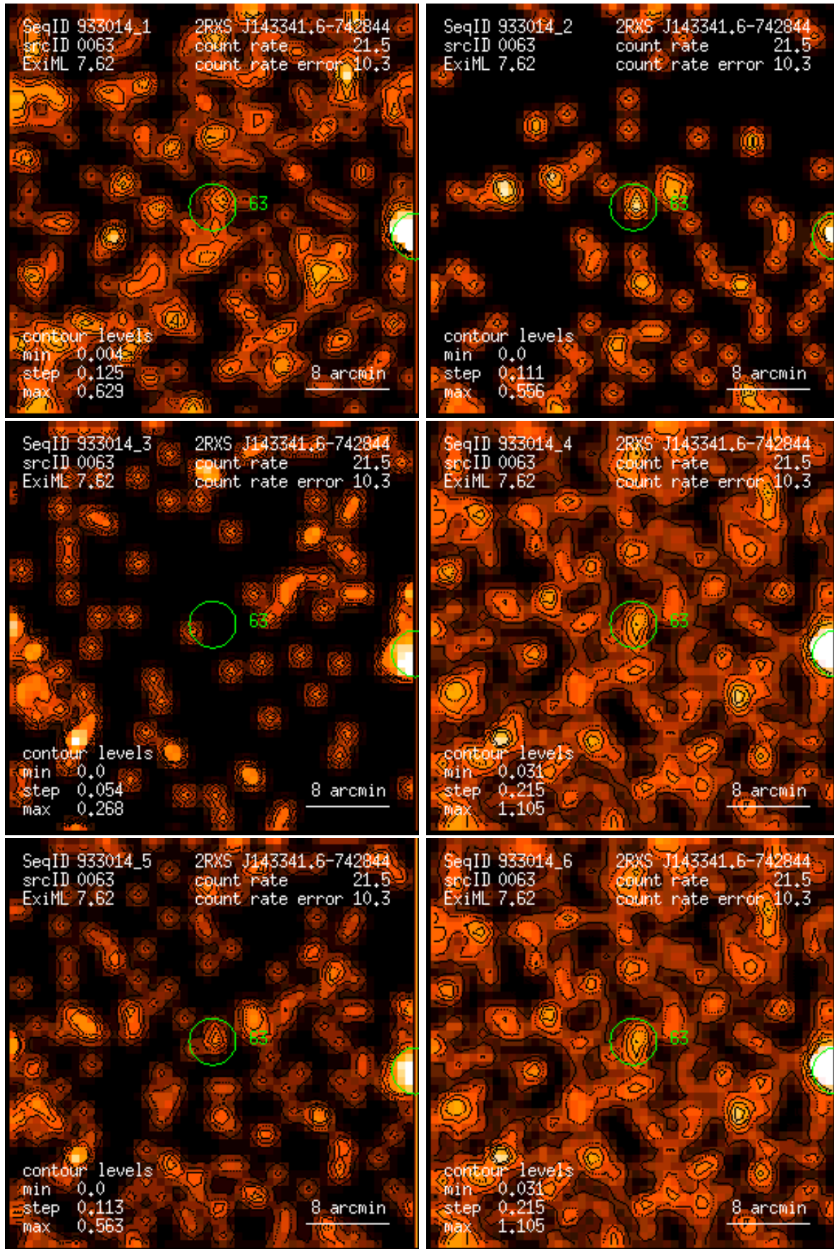
Figure 63: RASS 933014: detection 0063: band rate images, Gaussian filter: (1) PSPC channels 11 – 41, (2) 52 – 90, (3) 91 – 201, (4) 11 – 235, (5) 52 – 201, (6) 11 – 201. Broad band rates in counts/ks. Band rate contour levels in counts/ks/arcmin 2 .
