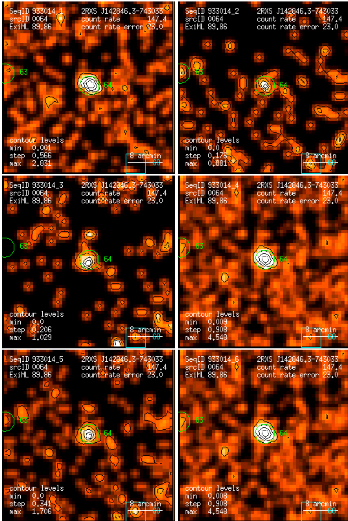
Figure 64: RASS 933014: detection 0064: band rate images, Gaussian filter: (1) PSPC channels 11 – 41, (2) 52 – 90, (3) 91 – 201, (4) 11 – 235, (5) 52 – 201, (6) 11 – 201. Broad band rates in counts/ks. Band rate contour levels in counts/ks/arcmin 2 .
