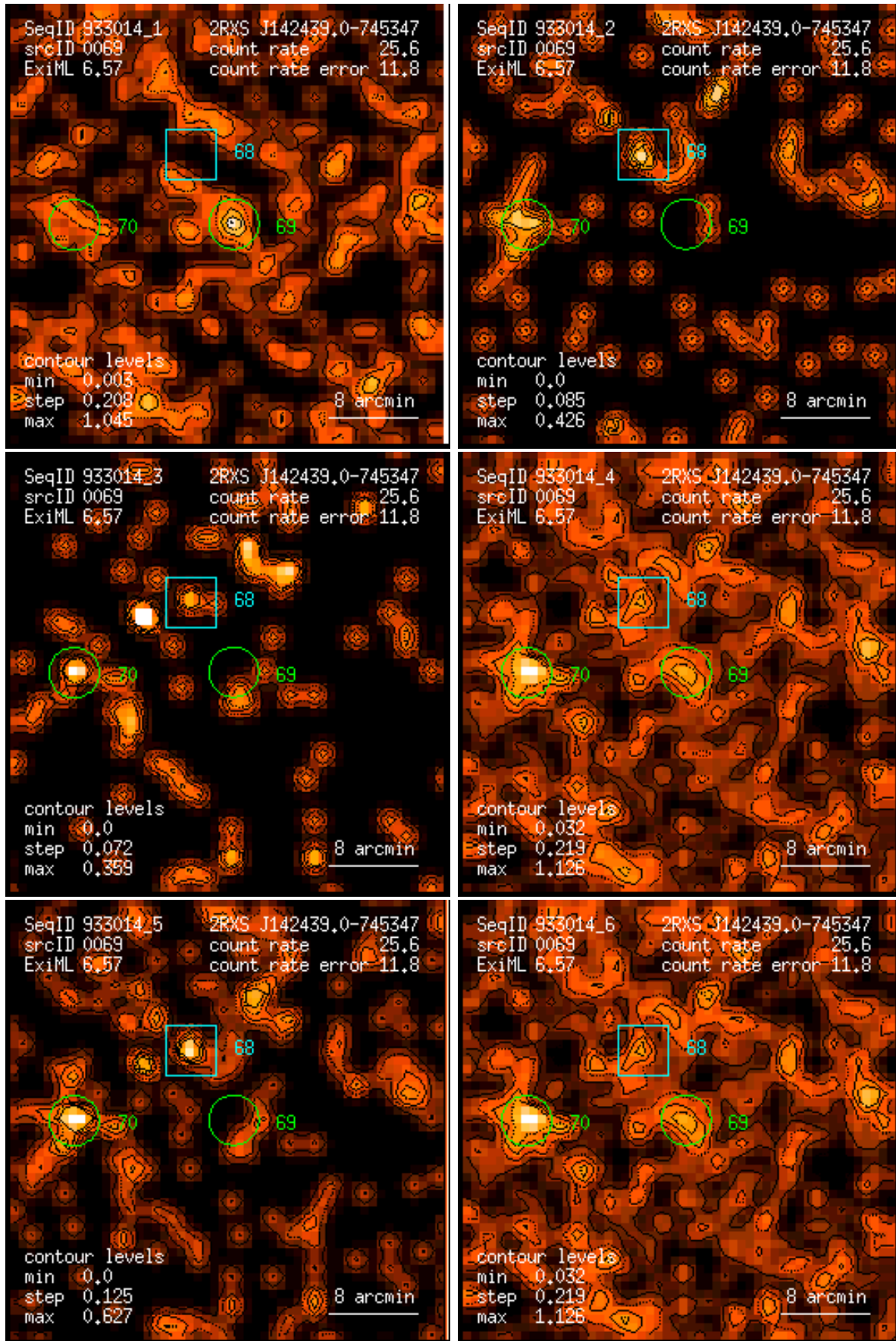
Figure 69: RASS 933014: detection 0069: band rate images, Gaussian filter: (1) PSPC channels 11 – 41, (2) 52 – 90, (3) 91 – 201, (4) 11 – 235, (5) 52 – 201, (6) 11 – 201. Broad band rates in counts/ks. Band rate contour levels in counts/ks/arcmin 2 .
