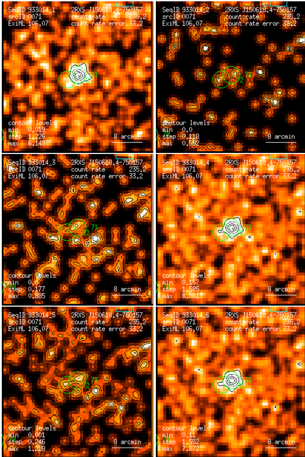
Figure 71: RASS 933014: detection 0071: band rate images, Gaussian filter: (1) PSPC channels 11 – 41, (2) 52 – 90, (3) 91 – 201, (4) 11 – 235, (5) 52 – 201, (6) 11 – 201. Broad band rates in counts/ks. Band rate contour levels in counts/ks/arcmin 2 .
