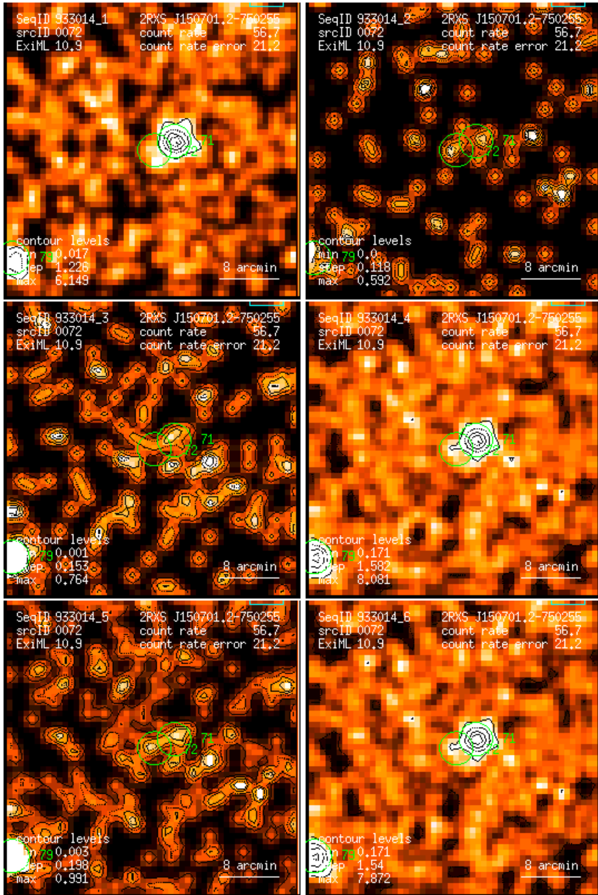
Figure 72: RASS 933014: detection 0072: band rate images, Gaussian filter: (1) PSPC channels 11 – 41, (2) 52 – 90, (3) 91 – 201, (4) 11 – 235, (5) 52 – 201, (6) 11 – 201. Broad band rates in counts/ks. Band rate contour levels in counts/ks/arcmin 2 .
