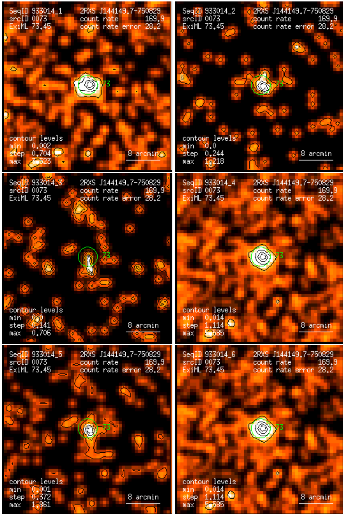
Figure 73: RASS 933014: detection 0073: band rate images, Gaussian filter: (1) PSPC channels 11 – 41, (2) 52 – 90, (3) 91 – 201, (4) 11 – 235, (5) 52 – 201, (6) 11 – 201. Broad band rates in counts/ks. Band rate contour levels in counts/ks/arcmin 2 .
