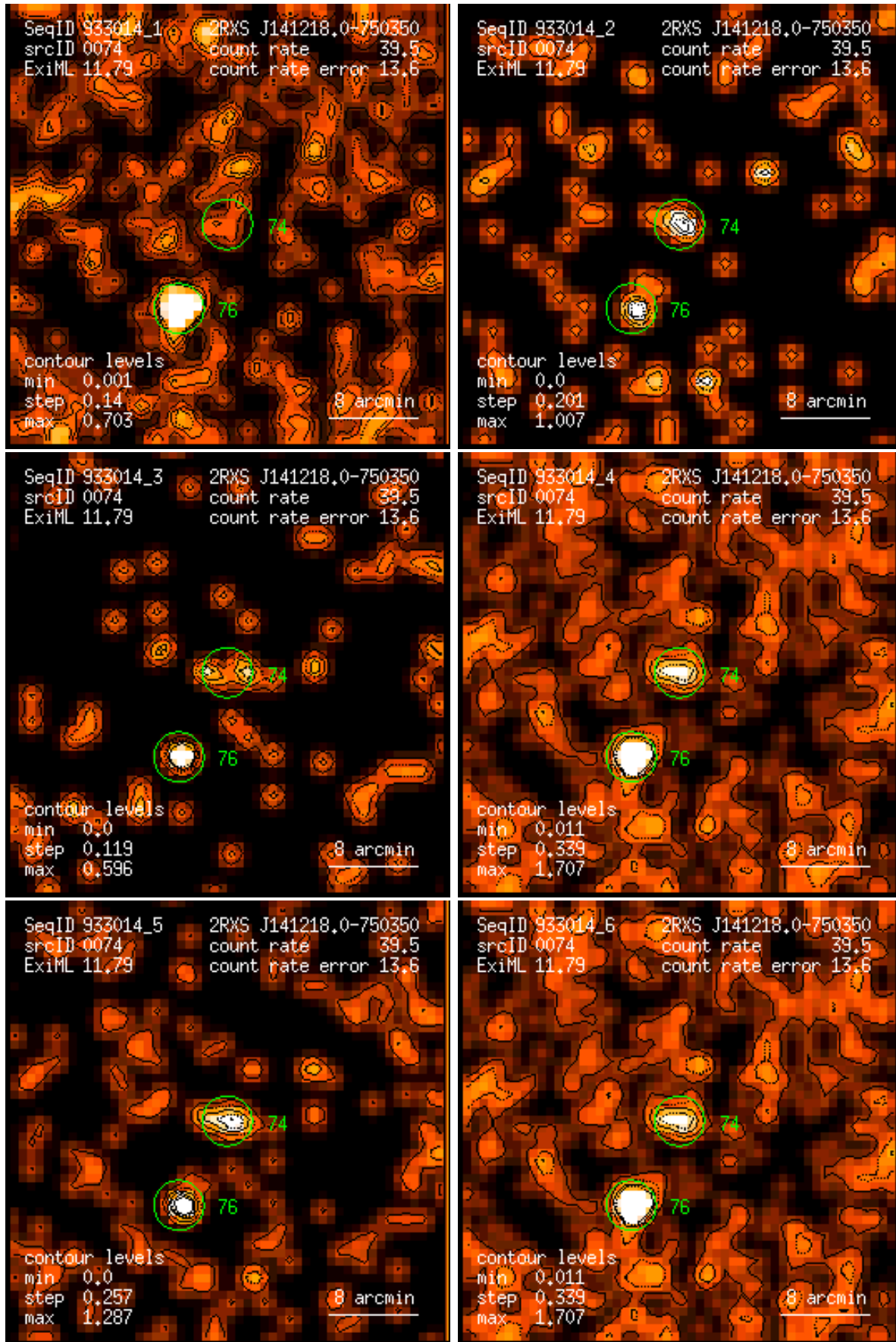
Figure 74: RASS 933014: detection 0074: band rate images, Gaussian filter: (1) PSPC channels 11 – 41, (2) 52 – 90, (3) 91 – 201, (4) 11 – 235, (5) 52 – 201, (6) 11 – 201. Broad band rates in counts/ks. Band rate contour levels in counts/ks/arcmin 2 .
