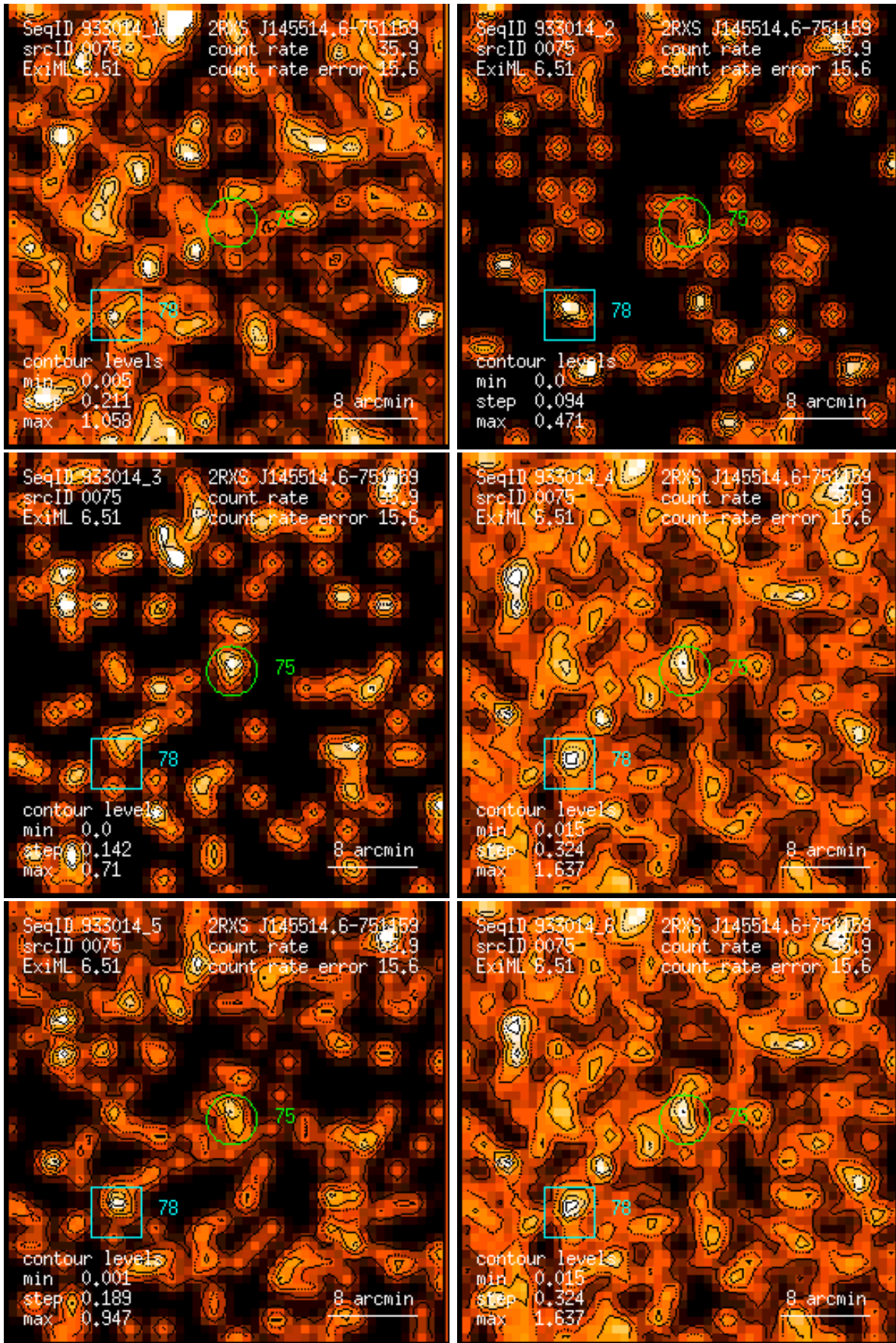
Figure 75: RASS 933014: detection 0075: band rate images, Gaussian filter: (1) PSPC channels 11 – 41, (2) 52 – 90, (3) 91 – 201, (4) 11 – 235, (5) 52 – 201, (6) 11 – 201. Broad band rates in counts/ks. Band rate contour levels in counts/ks/arcmin 2 .
