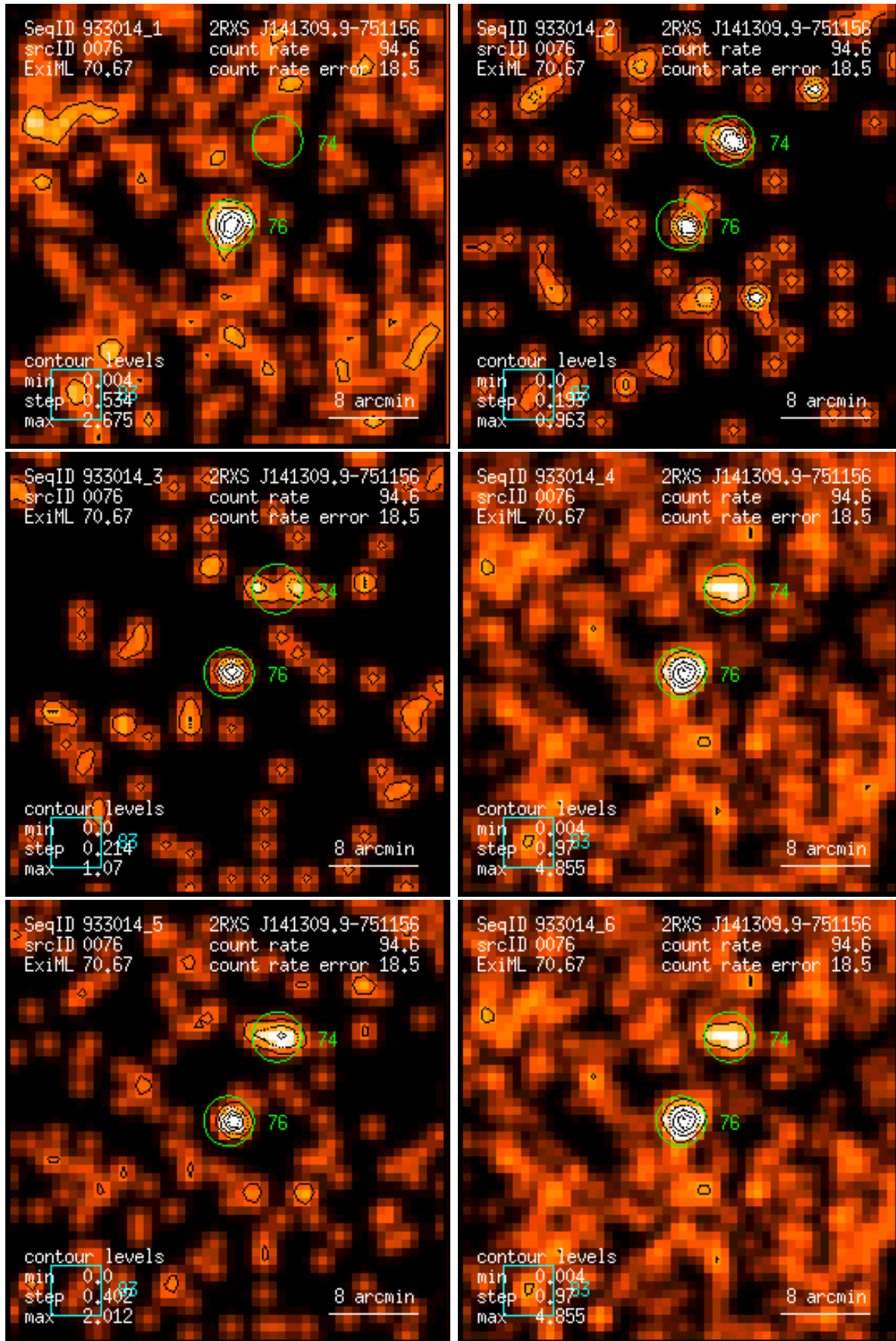
Figure 76: RASS 933014: detection 0076: band rate images, Gaussian filter: (1) PSPC channels 11 – 41, (2) 52 – 90, (3) 91 – 201, (4) 11 – 235, (5) 52 – 201, (6) 11 – 201. Broad band rates in counts/ks. Band rate contour levels in counts/ks/arcmin 2 .
