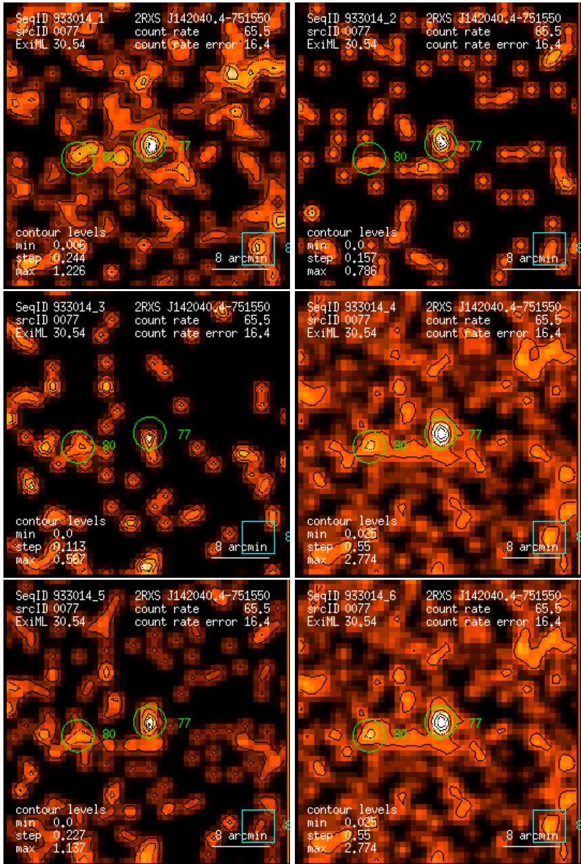
Figure 77: RASS 933014: detection 0077: band rate images, Gaussian filter: (1) PSPC channels 11 – 41, (2) 52 – 90, (3) 91 – 201, (4) 11 – 235, (5) 52 – 201, (6) 11 – 201. Broad band rates in counts/ks. Band rate contour levels in counts/ks/arcmin 2 .
