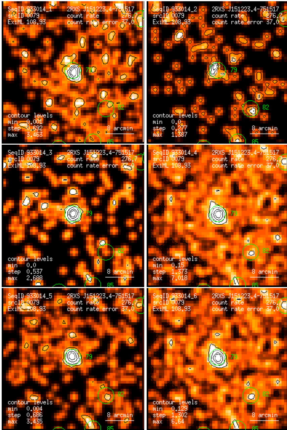
Figure 79: RASS 933014: detection 0079: band rate images, Gaussian filter: (1) PSPC channels 11 – 41, (2) 52 – 90, (3) 91 – 201, (4) 11 – 235, (5) 52 – 201, (6) 11 – 201. Broad band rates in counts/ks. Band rate contour levels in counts/ks/arcmin 2 .
