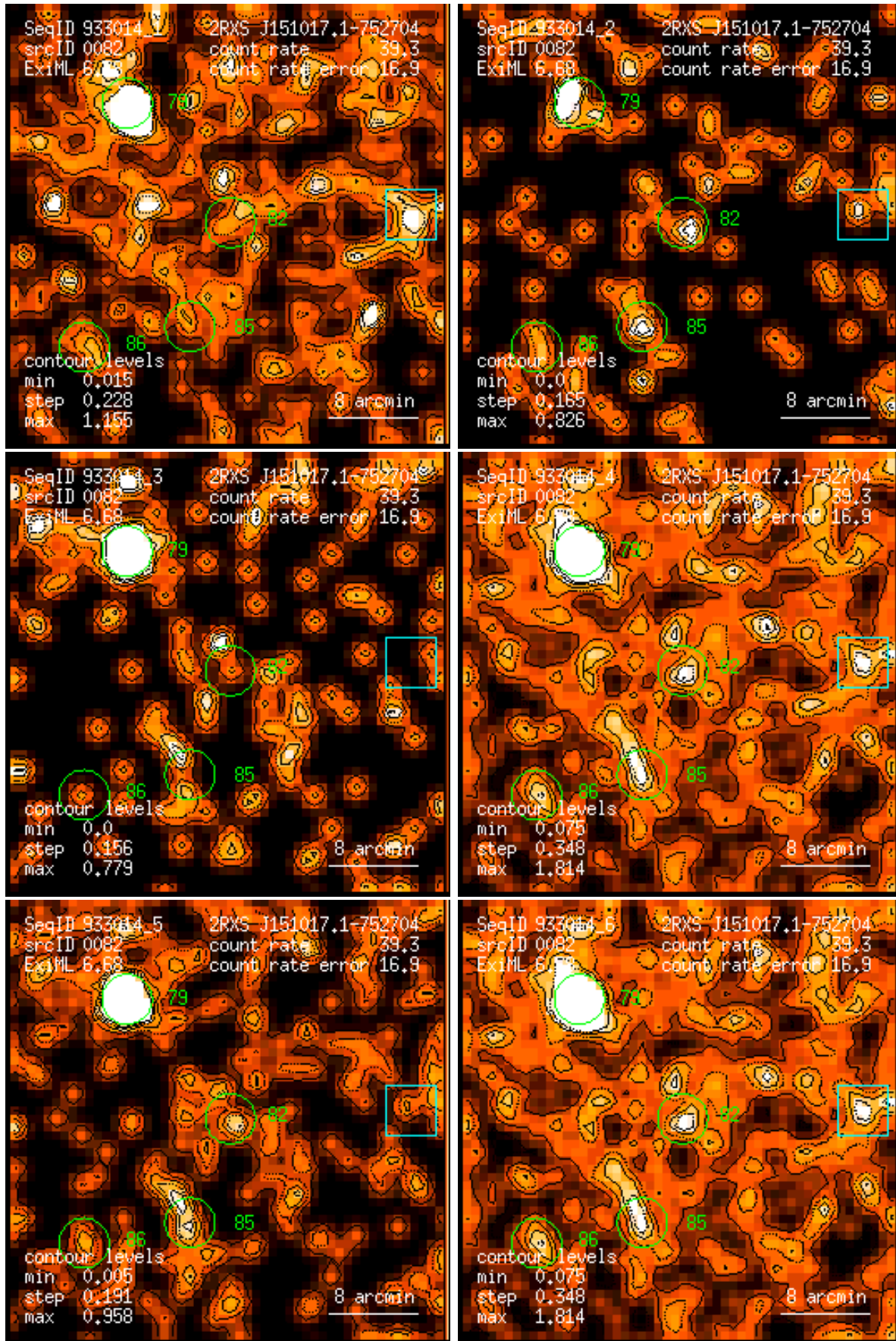
Figure 82: RASS 933014: detection 0082: band rate images, Gaussian filter: (1) PSPC channels 11 – 41, (2) 52 – 90, (3) 91 – 201, (4) 11 – 235, (5) 52 – 201, (6) 11 – 201. Broad band rates in counts/ks. Band rate contour levels in counts/ks/arcmin 2 .
