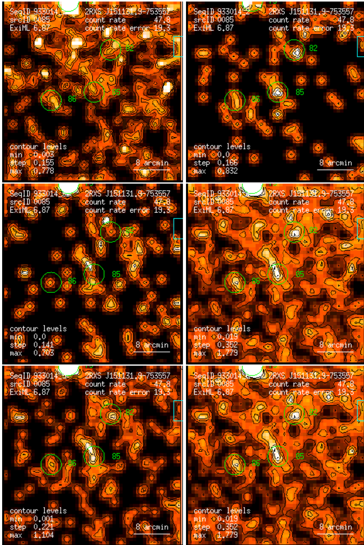
Figure 85: RASS 933014: detection 0085: band rate images, Gaussian filter: (1) PSPC channels 11 – 41, (2) 52 – 90, (3) 91 – 201, (4) 11 – 235, (5) 52 – 201, (6) 11 – 201. Broad band rates in counts/ks. Band rate contour levels in counts/ks/arcmin 2 .
