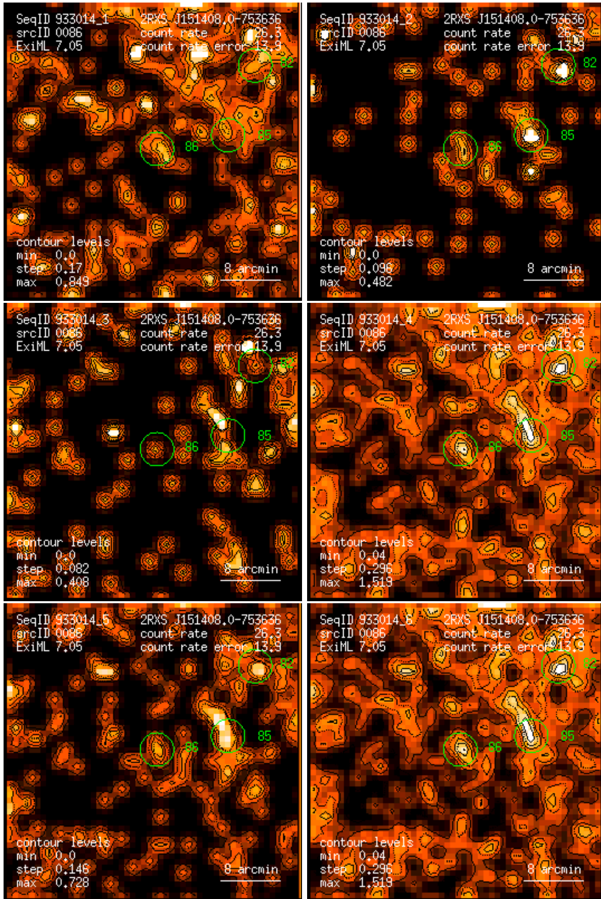
Figure 86: RASS 933014: detection 0086: band rate images, Gaussian filter: (1) PSPC channels 11 – 41, (2) 52 – 90, (3) 91 – 201, (4) 11 – 235, (5) 52 – 201, (6) 11 – 201. Broad band rates in counts/ks. Band rate contour levels in counts/ks/arcmin 2 .
