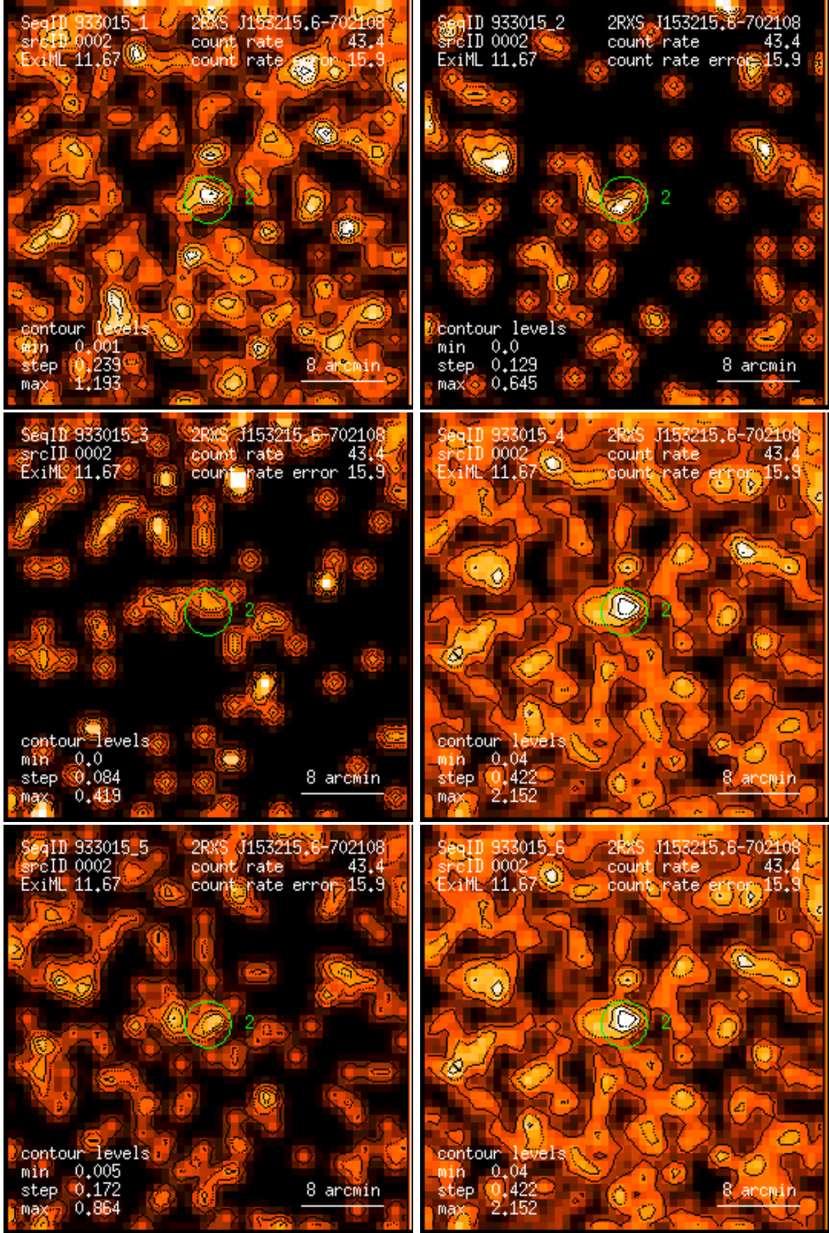
Figure 2: RASS 933015: detection 0002: band rate images, Gaussian filter: (1) PSPC channels 11 – 41, (2) 52 – 90, (3) 91 – 201, (4) 11 – 235, (5) 52 – 201, (6) 11 – 201. Broad band rates in counts/ks. Band rate contour levels in counts/ks/arcmin 2 .
