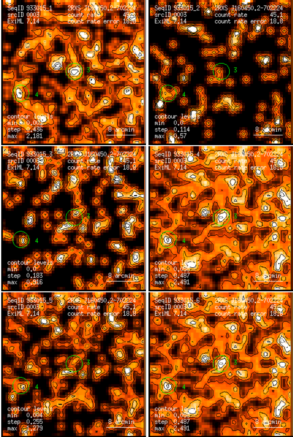
Figure 3: RASS 933015: detection 0003: band rate images, Gaussian filter: (1) PSPC channels 11 – 41, (2) 52 – 90, (3) 91 – 201, (4) 11 – 235, (5) 52 – 201, (6) 11 – 201. Broad band rates in counts/ks. Band rate contour levels in counts/ks/arcmin 2 .
