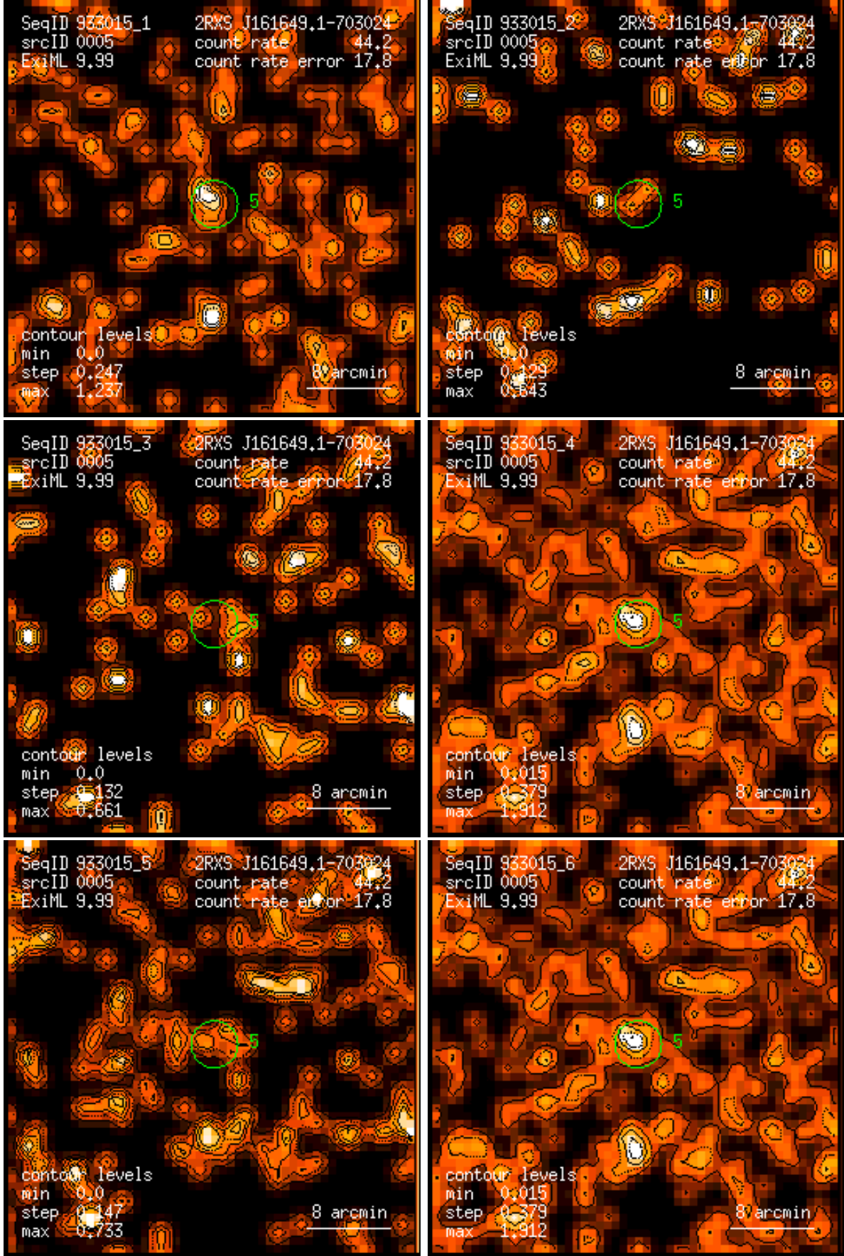
Figure 5: RASS 933015: detection 0005: band rate images, Gaussian filter: (1) PSPC channels 11 – 41, (2) 52 – 90, (3) 91 – 201, (4) 11 – 235, (5) 52 – 201, (6) 11 – 201. Broad band rates in counts/ks. Band rate contour levels in counts/ks/arcmin 2 .
