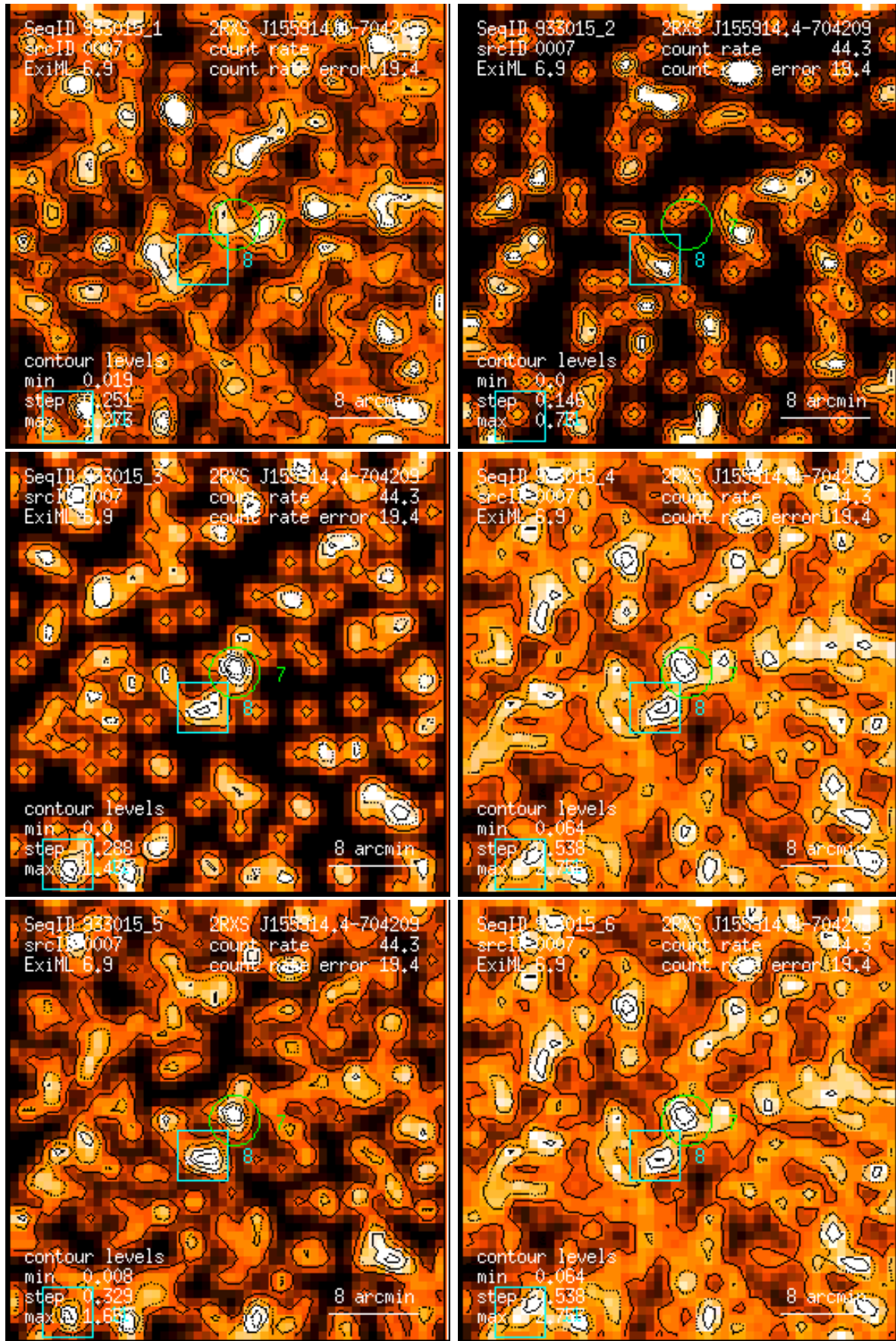
Figure 7: RASS 933015: detection 0007: band rate images, Gaussian filter: (1) PSPC channels 11 – 41, (2) 52 – 90, (3) 91 – 201, (4) 11 – 235, (5) 52 – 201, (6) 11 – 201. Broad band rates in counts/ks. Band rate contour levels in counts/ks/arcmin 2 .
