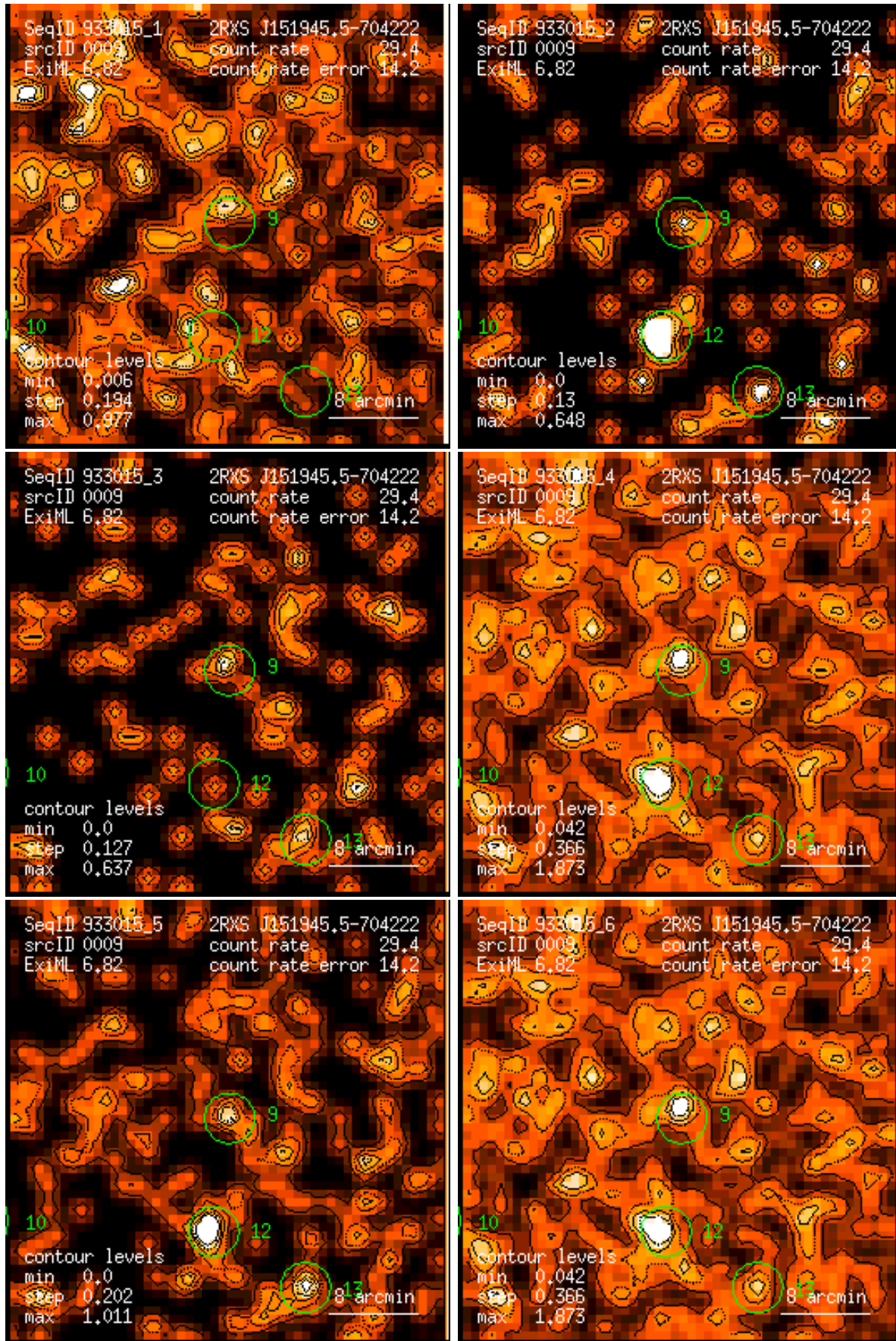
Figure 9: RASS 933015: detection 0009: band rate images, Gaussian filter: (1) PSPC channels 11 – 41, (2) 52 – 90, (3) 91 – 201, (4) 11 – 235, (5) 52 – 201, (6) 11 – 201. Broad band rates in counts/ks. Band rate contour levels in counts/ks/arcmin 2 .
