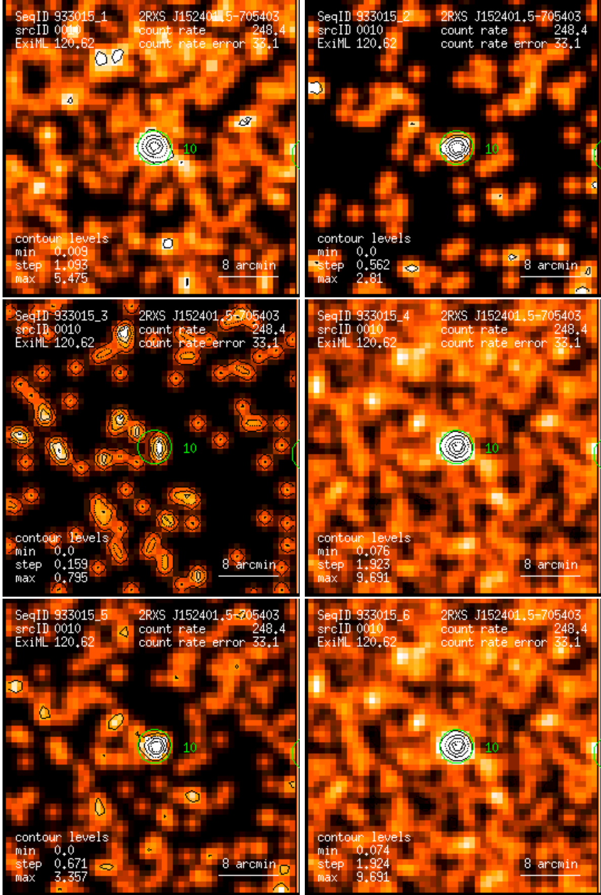
Figure 10: RASS 933015: detection 0010: band rate images, Gaussian filter: (1) PSPC channels 11 – 41, (2) 52 – 90, (3) 91 – 201, (4) 11 – 235, (5) 52 – 201, (6) 11 – 201. Broad band rates in counts/ks. Band rate contour levels in counts/ks/arcmin 2 .
