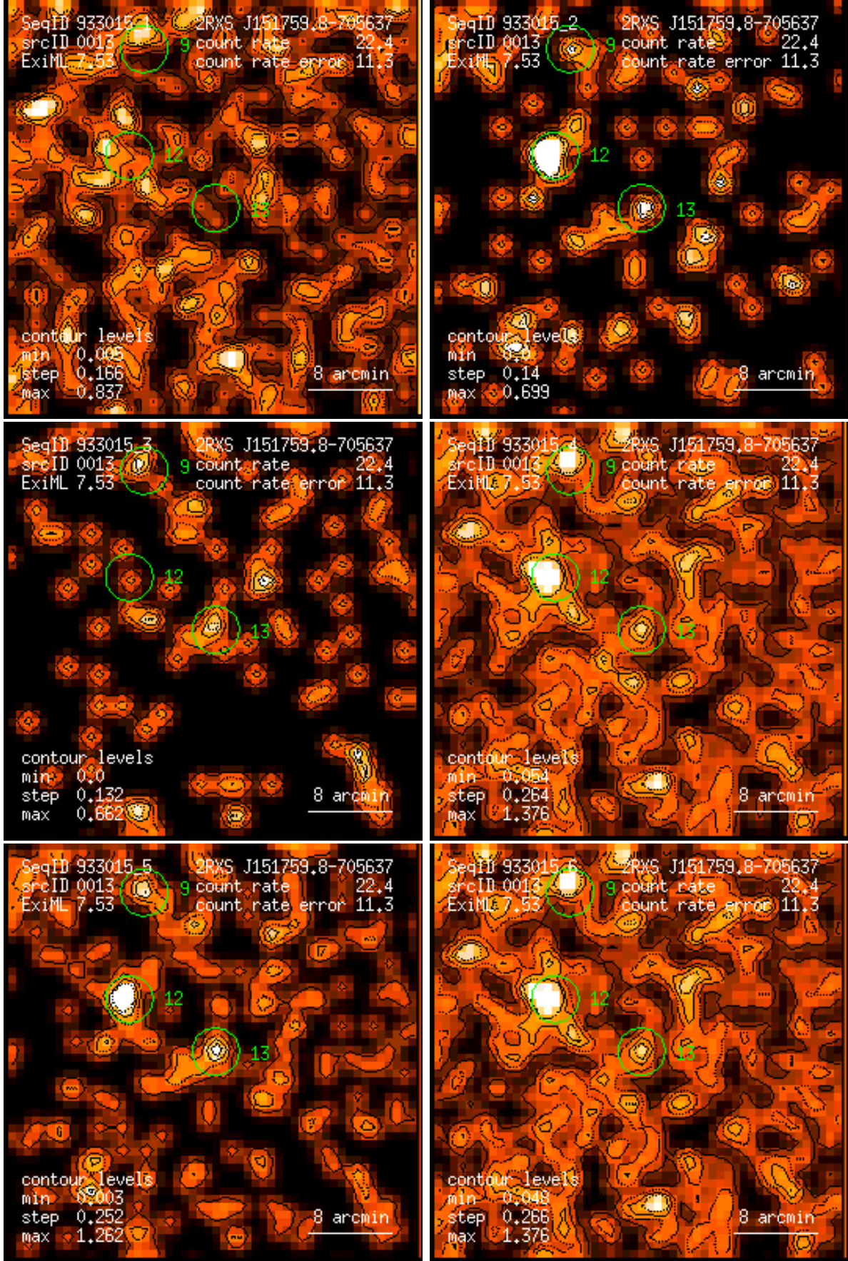
Figure 13: RASS 933015: detection 0013: band rate images, Gaussian filter: (1) PSPC channels 11 – 41, (2) 52 – 90, (3) 91 – 201, (4) 11 – 235, (5) 52 – 201, (6) 11 – 201. Broad band rates in counts/ks. Band rate contour levels in counts/ks/arcmin 2 .
