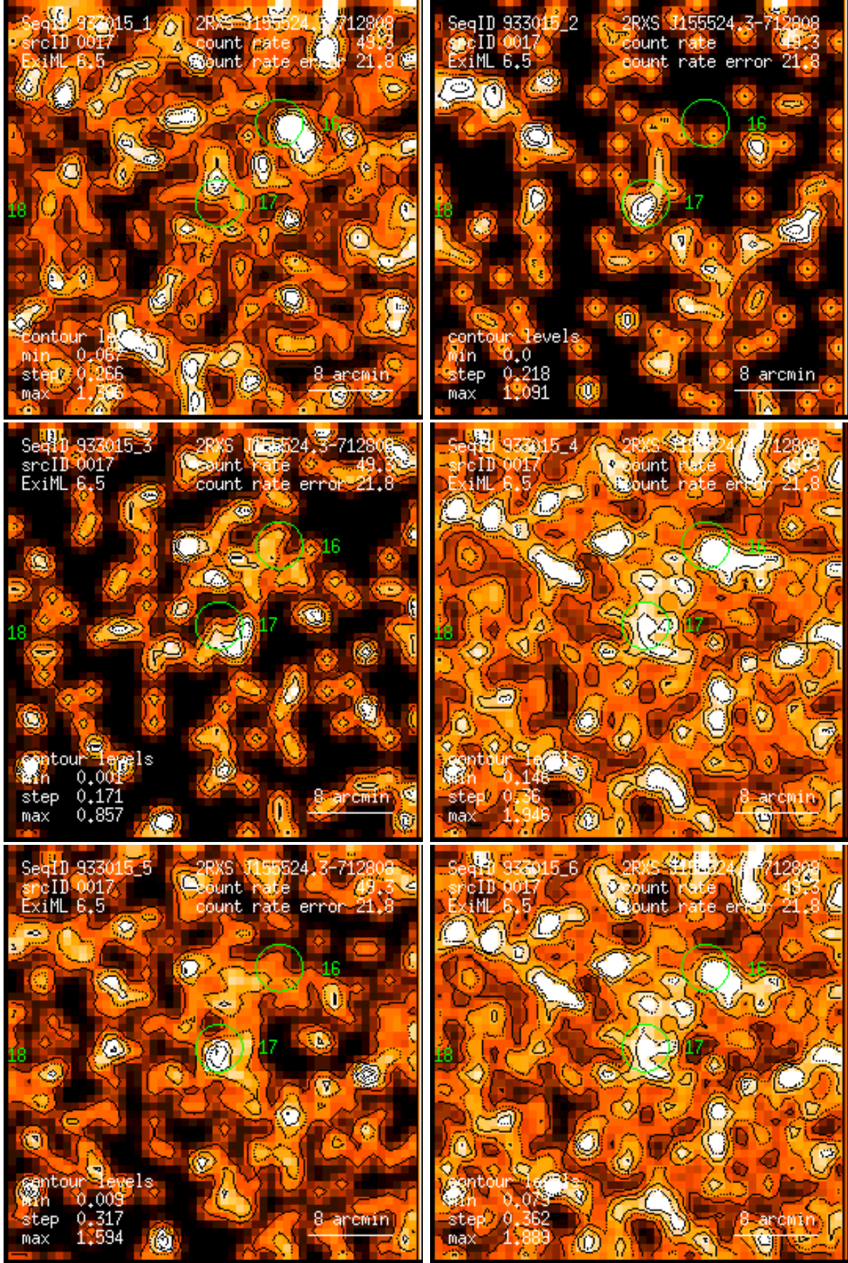
Figure 17: RASS 933015: detection 0017: band rate images, Gaussian filter: (1) PSPC channels 11 – 41, (2) 52 – 90, (3) 91 – 201, (4) 11 – 235, (5) 52 – 201, (6) 11 – 201. Broad band rates in counts/ks. Band rate contour levels in counts/ks/arcmin 2 .
