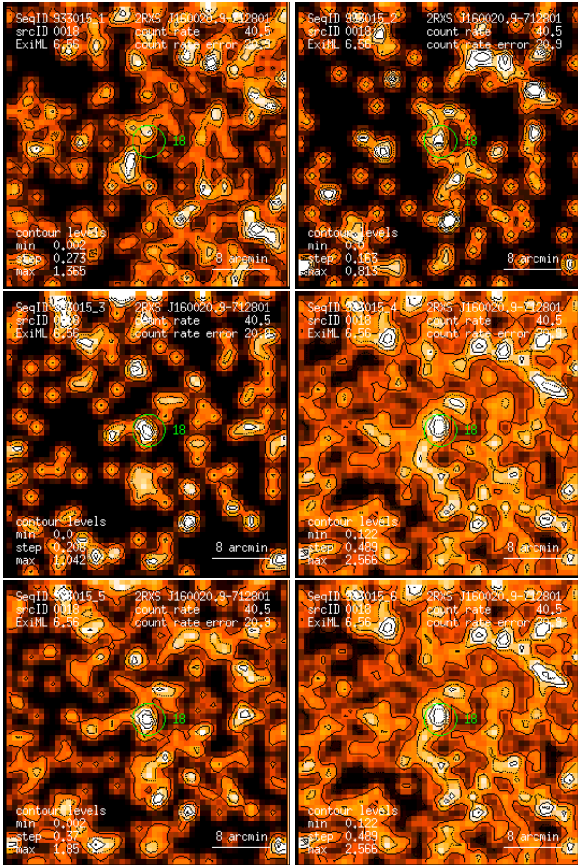
Figure 18: RASS 933015: detection 0018: band rate images, Gaussian filter: (1) PSPC channels 11 – 41, (2) 52 – 90, (3) 91 – 201, (4) 11 – 235, (5) 52 – 201, (6) 11 – 201. Broad band rates in counts/ks. Band rate contour levels in counts/ks/arcmin 2 .
