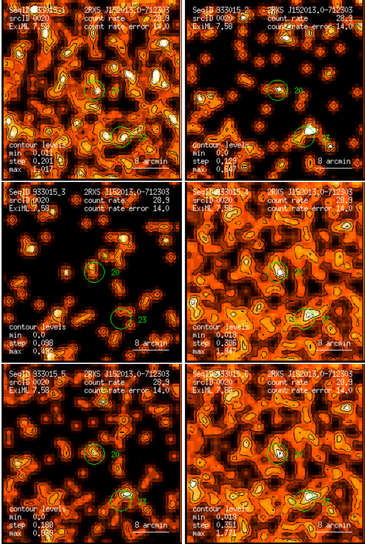
Figure 20: RASS 933015: detection 0020: band rate images, Gaussian filter: (1) PSPC channels 11 – 41, (2) 52 – 90, (3) 91 – 201, (4) 11 – 235, (5) 52 – 201, (6) 11 – 201. Broad band rates in counts/ks. Band rate contour levels in counts/ks/arcmin 2 .
