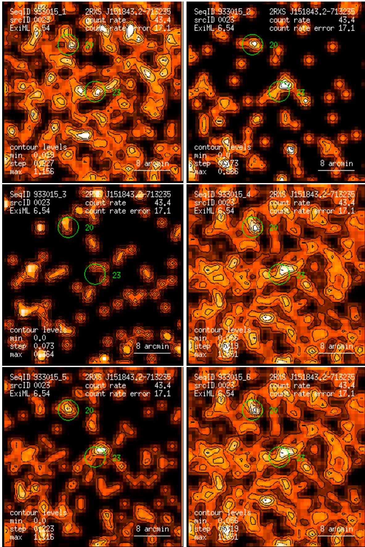
Figure 23: RASS 933015: detection 0023: band rate images, Gaussian filter: (1) PSPC channels 11 – 41, (2) 52 – 90, (3) 91 – 201, (4) 11 – 235, (5) 52 – 201, (6) 11 – 201. Broad band rates in counts/ks. Band rate contour levels in counts/ks/arcmin 2 .
