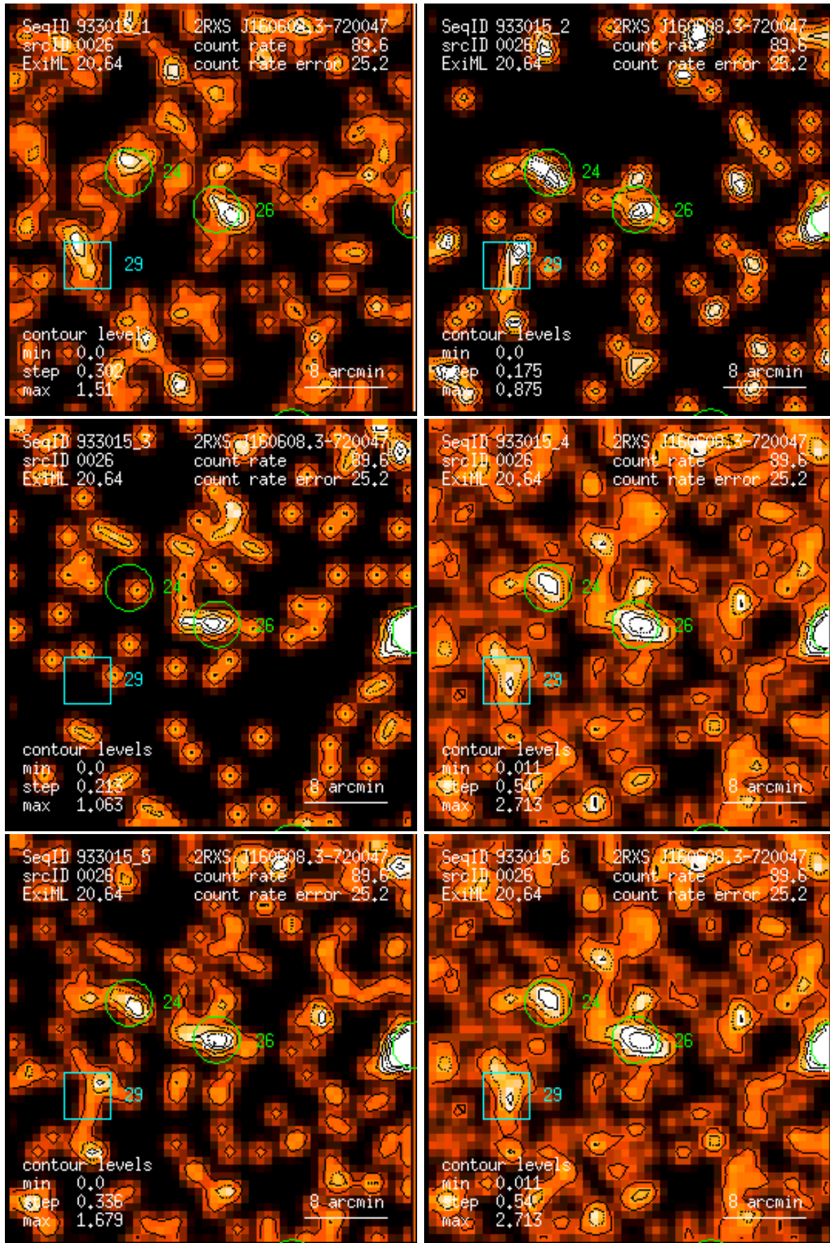
Figure 26: RASS 933015: detection 0026: band rate images, Gaussian filter: (1) PSPC channels 11 – 41, (2) 52 – 90, (3) 91 – 201, (4) 11 – 235, (5) 52 – 201, (6) 11 – 201. Broad band rates in counts/ks. Band rate contour levels in counts/ks/arcmin 2 .
