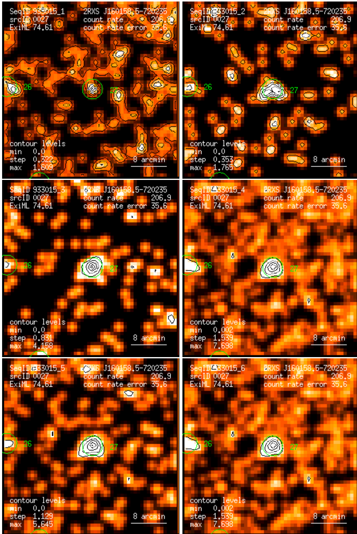
Figure 27: RASS 933015: detection 0027: band rate images, Gaussian filter: (1) PSPC channels 11 – 41, (2) 52 – 90, (3) 91 – 201, (4) 11 – 235, (5) 52 – 201, (6) 11 – 201. Broad band rates in counts/ks. Band rate contour levels in counts/ks/arcmin 2 .
