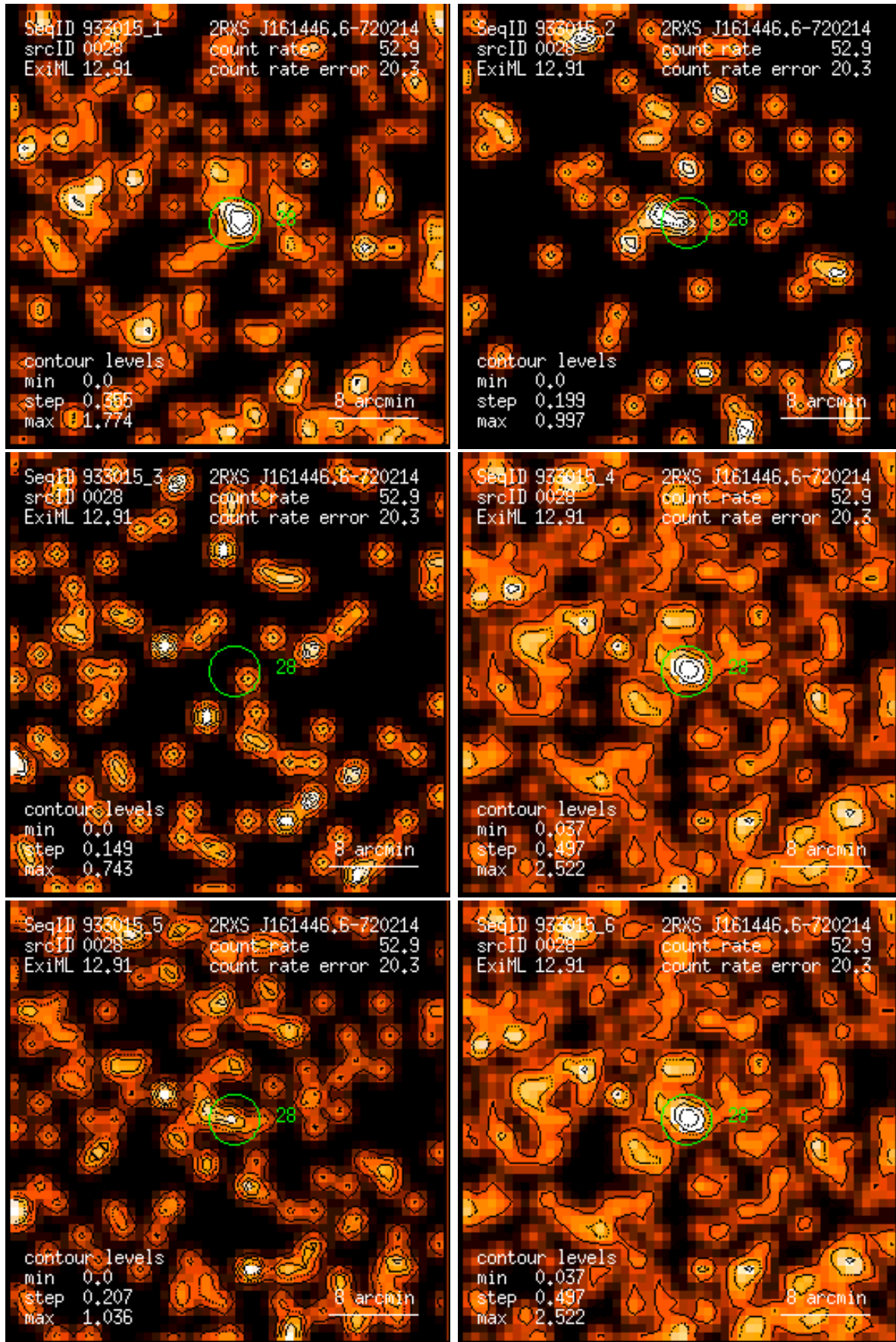
Figure 28: RASS 933015: detection 0028: band rate images, Gaussian filter: (1) PSPC channels 11 – 41, (2) 52 – 90, (3) 91 – 201, (4) 11 – 235, (5) 52 – 201, (6) 11 – 201. Broad band rates in counts/ks. Band rate contour levels in counts/ks/arcmin 2 .
