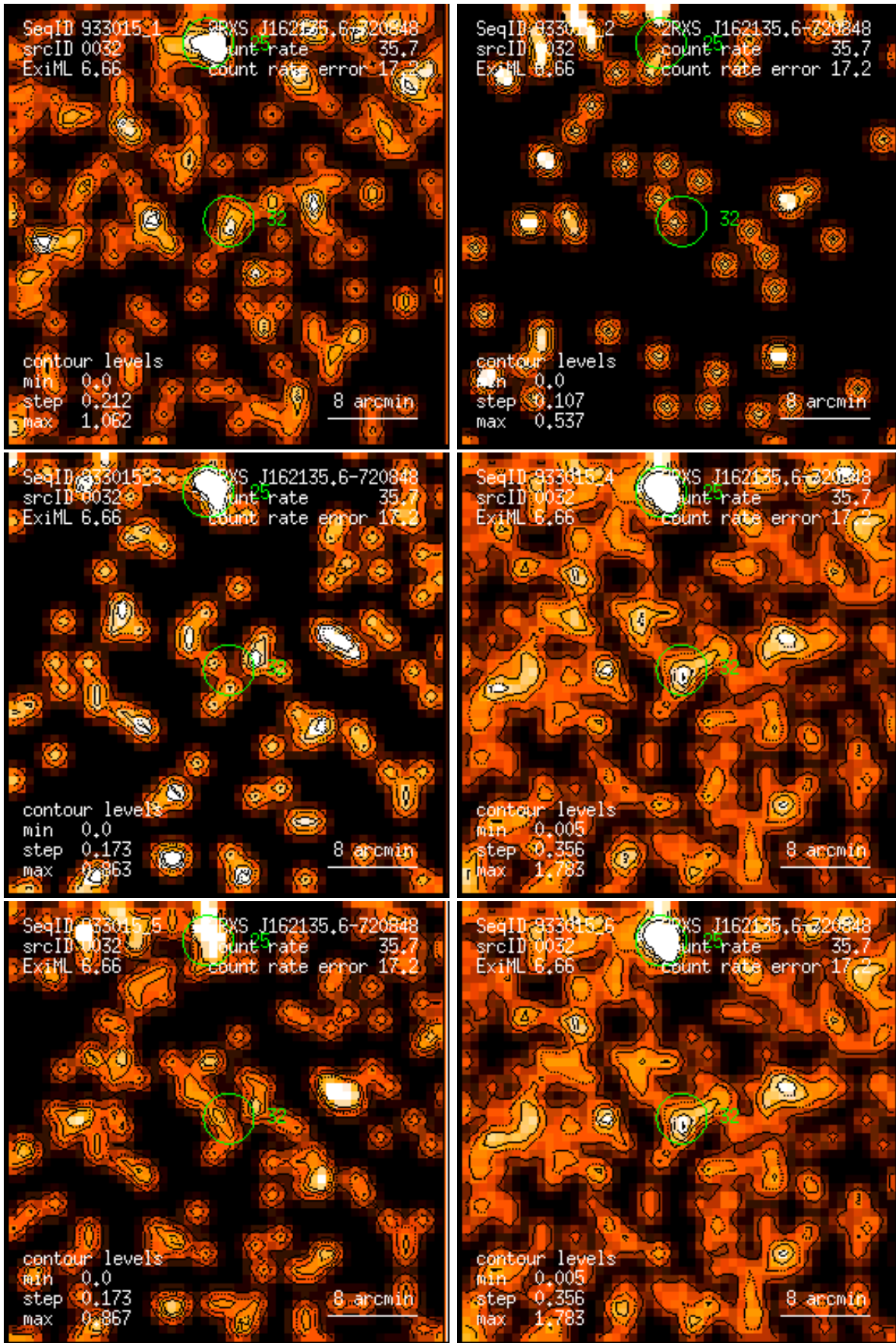
Figure 32: RASS 933015: detection 0032: band rate images, Gaussian filter: (1) PSPC channels 11 – 41, (2) 52 – 90, (3) 91 – 201, (4) 11 – 235, (5) 52 – 201, (6) 11 – 201. Broad band rates in counts/ks. Band rate contour levels in counts/ks/arcmin 2 .
