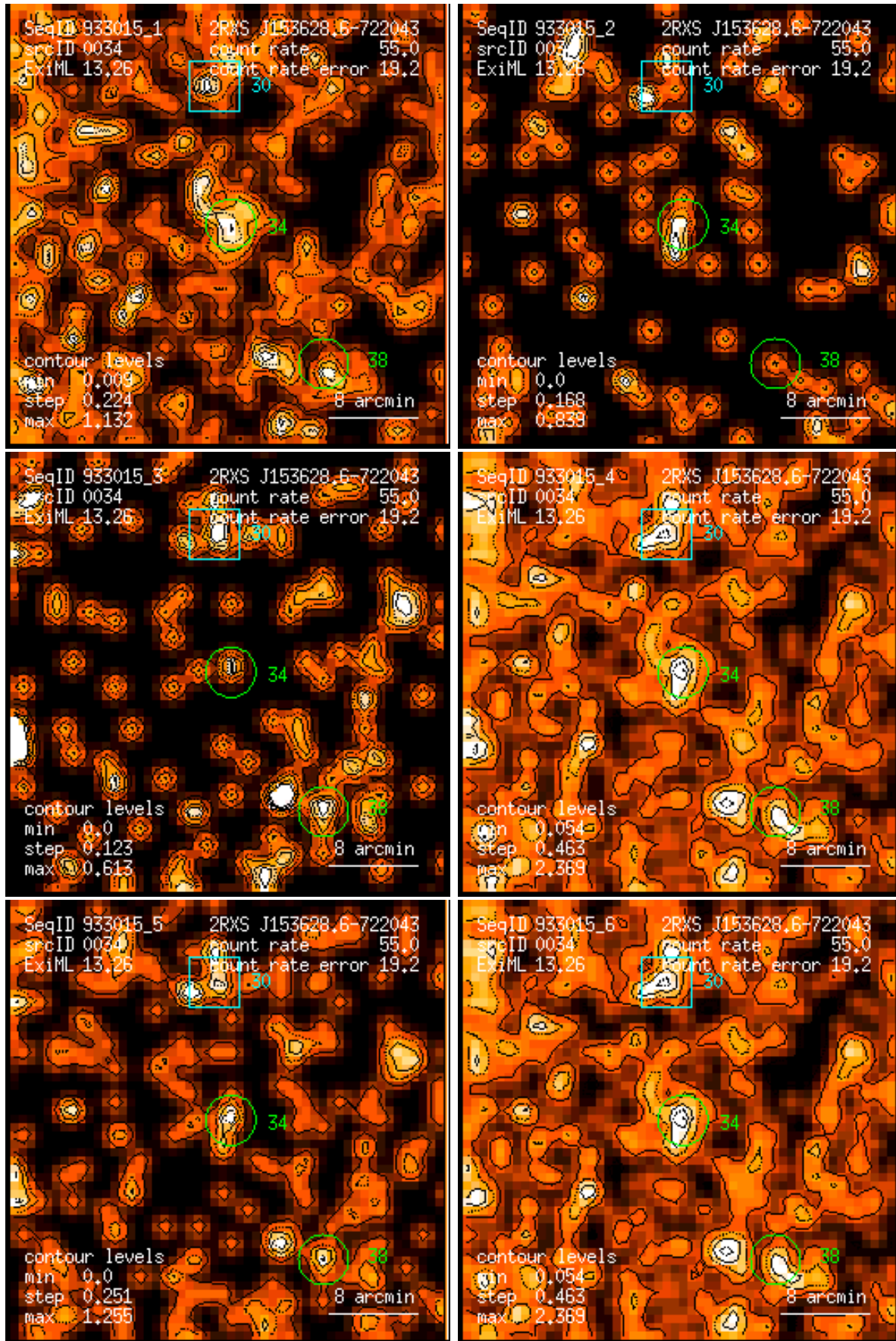
Figure 34: RASS 933015: detection 0034: band rate images, Gaussian filter: (1) PSPC channels 11 – 41, (2) 52 – 90, (3) 91 – 201, (4) 11 – 235, (5) 52 – 201, (6) 11 – 201. Broad band rates in counts/ks. Band rate contour levels in counts/ks/arcmin 2 .
