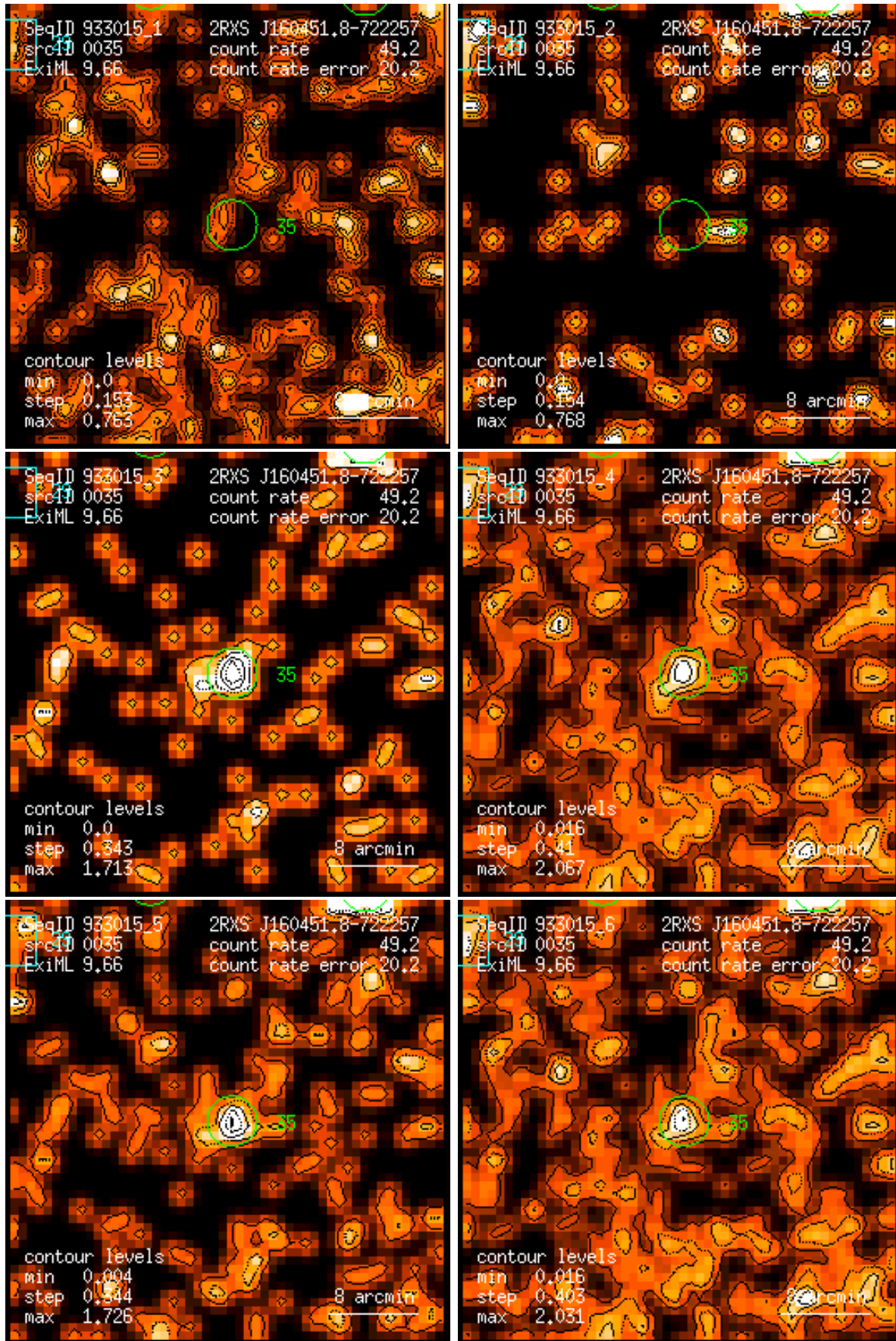
Figure 35: RASS 933015: detection 0035: band rate images, Gaussian filter: (1) PSPC channels 11 – 41, (2) 52 – 90, (3) 91 – 201, (4) 11 – 235, (5) 52 – 201, (6) 11 – 201. Broad band rates in counts/ks. Band rate contour levels in counts/ks/arcmin 2 .
