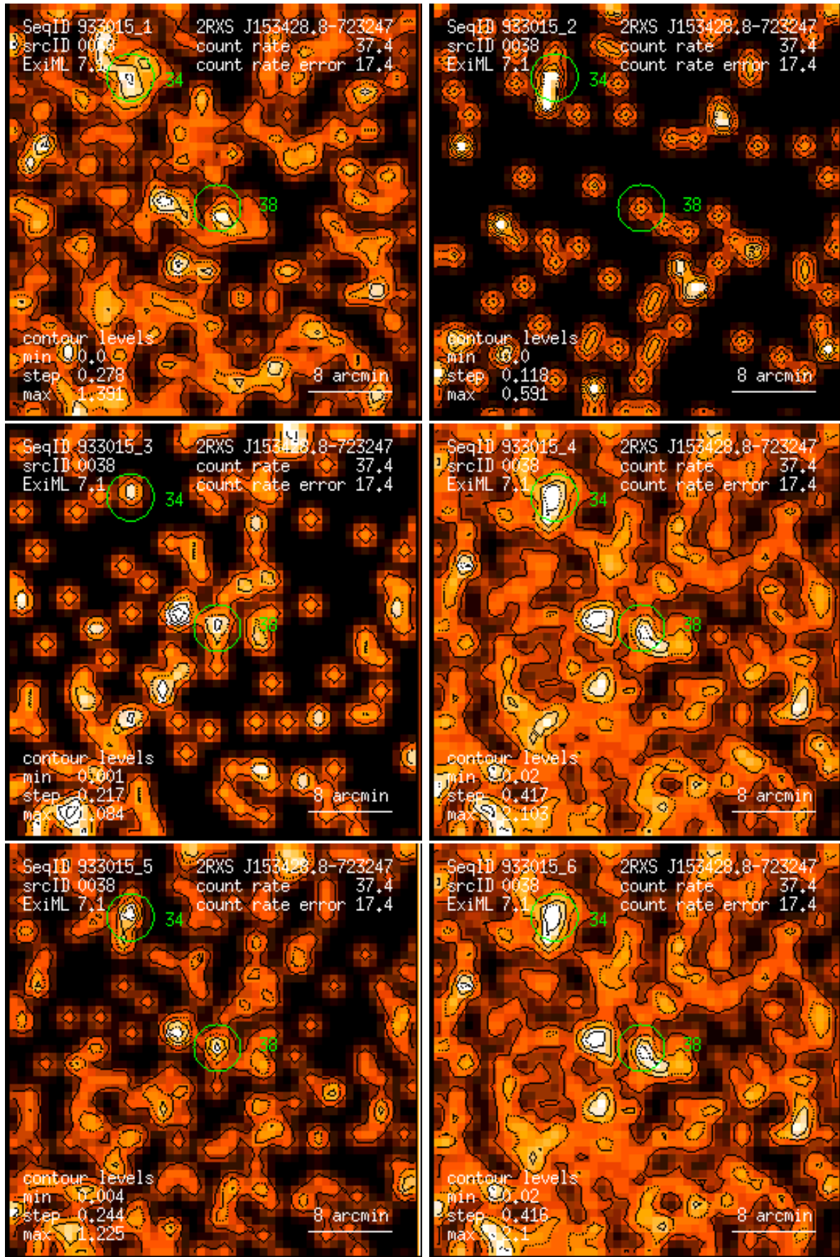
Figure 38: RASS 933015: detection 0038: band rate images, Gaussian filter: (1) PSPC channels 11 – 41, (2) 52 – 90, (3) 91 – 201, (4) 11 – 235, (5) 52 – 201, (6) 11 – 201. Broad band rates in counts/ks. Band rate contour levels in counts/ks/arcmin 2 .
