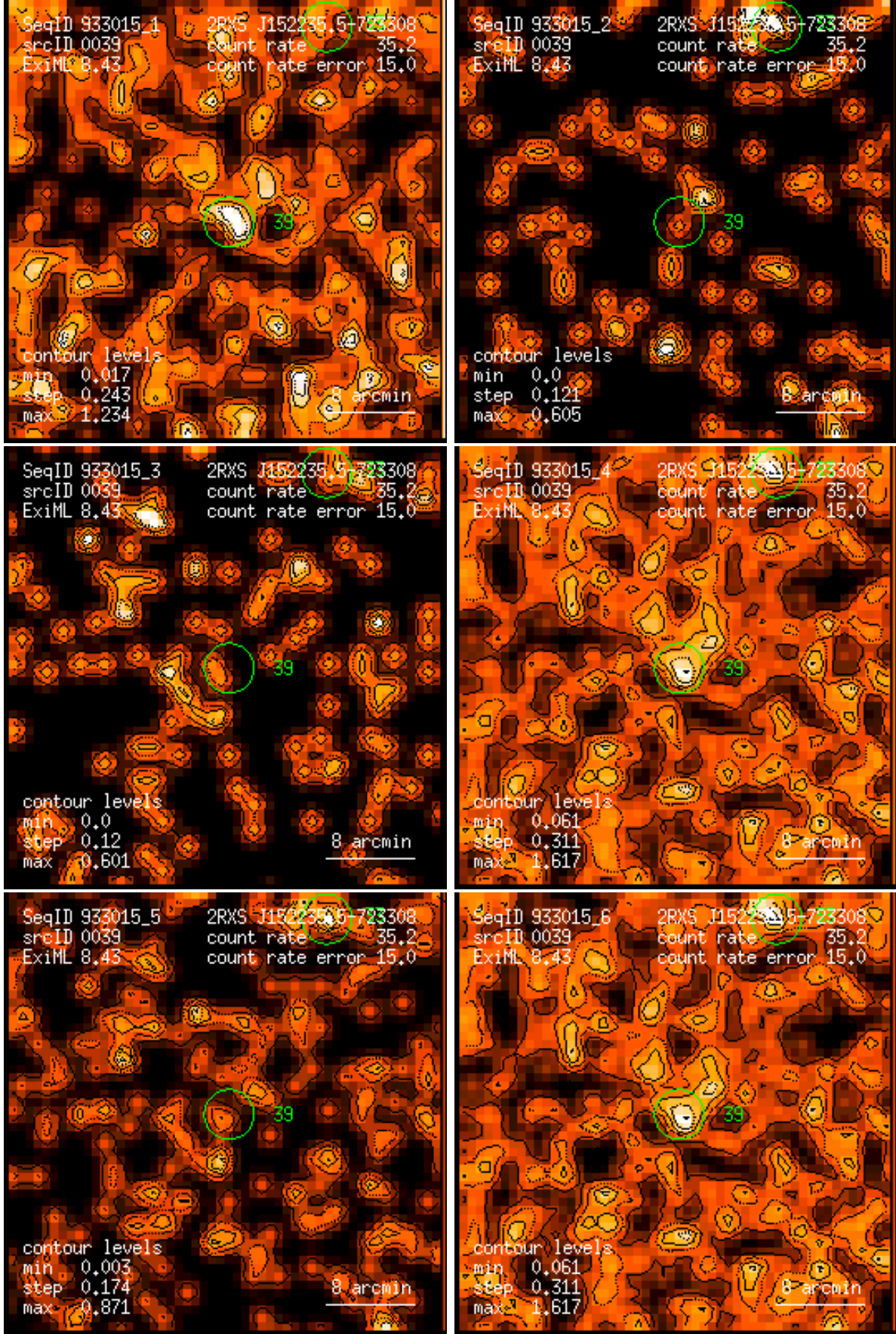
Figure 39: RASS 933015: detection 0039: band rate images, Gaussian filter: (1) PSPC channels 11 – 41, (2) 52 – 90, (3) 91 – 201, (4) 11 – 235, (5) 52 – 201, (6) 11 – 201. Broad band rates in counts/ks. Band rate contour levels in counts/ks/arcmin 2 .
